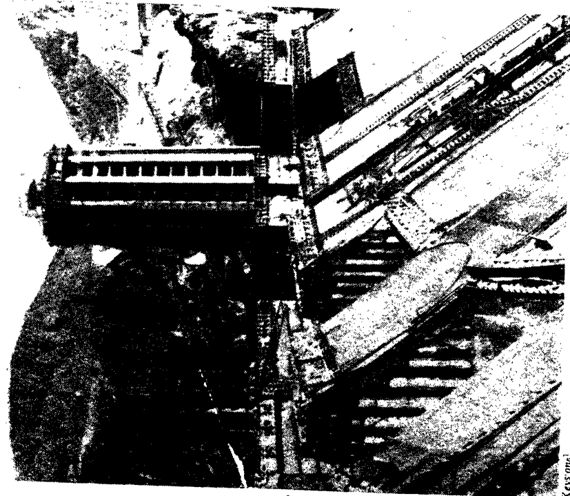
BUILDING THE COLORADO DAM The gigantic Boulder Dam is 554 feet high, and this picture shows its half-completed downstream face from the Nevada abutments. Two intakes for the huge power-plant at the base of the dam are shown towering above the mass of concrete. With the help of Hoop-lighting, construction work was carried on all night as well as all day.
