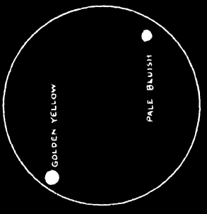
\beta LEONIS
