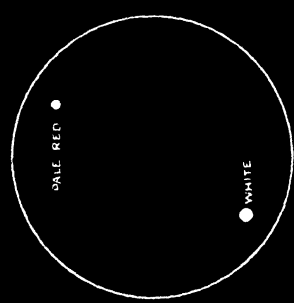
\beta CYGNI
