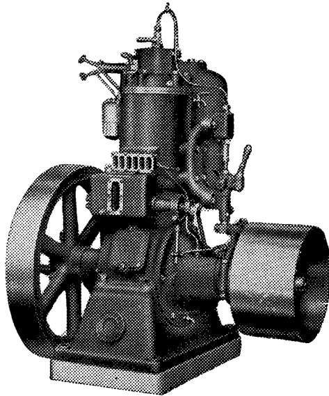
"DROTT" Crude Oil Engine.
