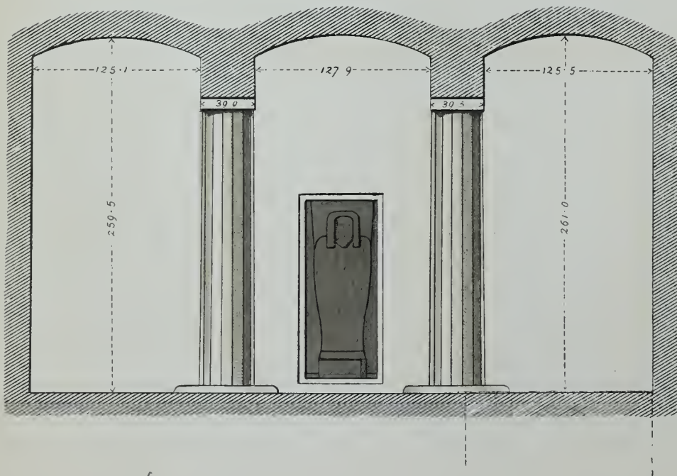
SECTIONAL ELEVATION ON C D.
