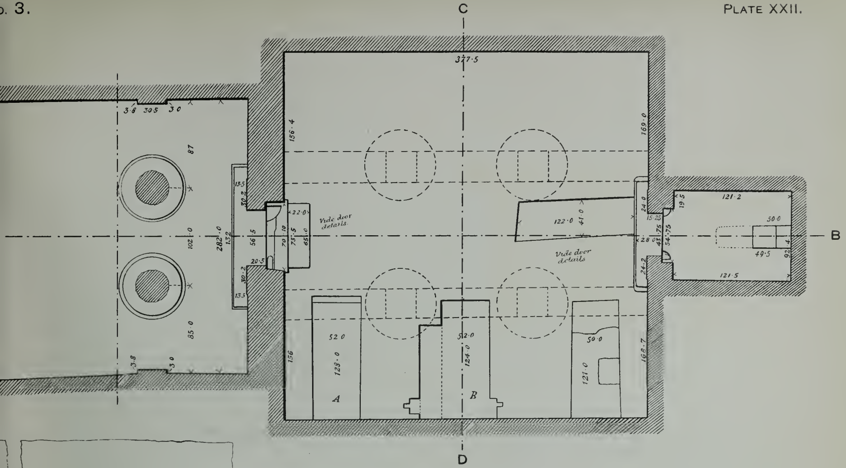
PLAN
