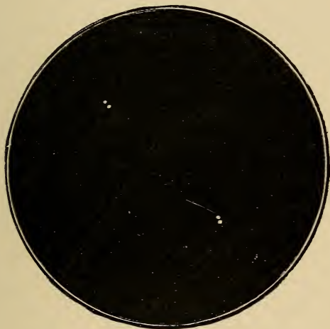
FIG. '19.—Quadruple star \epsilon of the Lyre.
