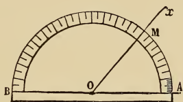
FIG. 80.—Measurement of Angles.
