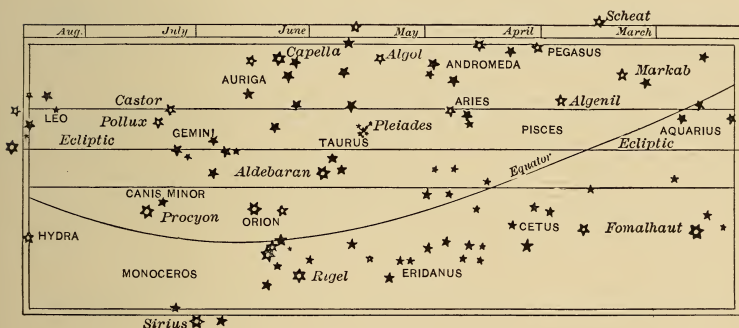
FIG. 11.—The Constellations of the Zodiac : winter and spring ; Crab, Twins, Bull, Ram, Fishes, Water-Carrier.
