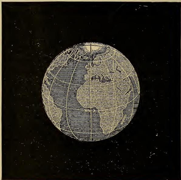
FIG. 2.—The earth in space. June solstice, midday.
