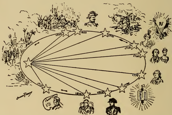
FIG. 27.—Stellar dial of the double star \gamma of the Virgin.
