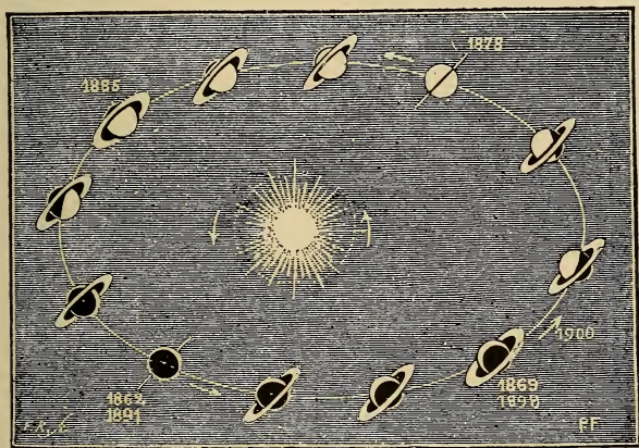
FIG. 48.—Varying perspective of Saturn's Rings, as seen from the Earth.
