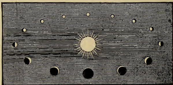
FIG. 37.—Successive phases of Venus.
