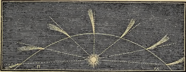
FIG. 53.—The tails of Comets are opposed to the Sun.
