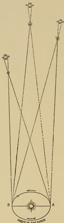
FIG. 84.—Small apparent ellipses described by the stars as a result of the annual displacement of the Earth.
