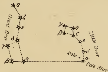
FIG. 4.—To find the Pole-Star.
