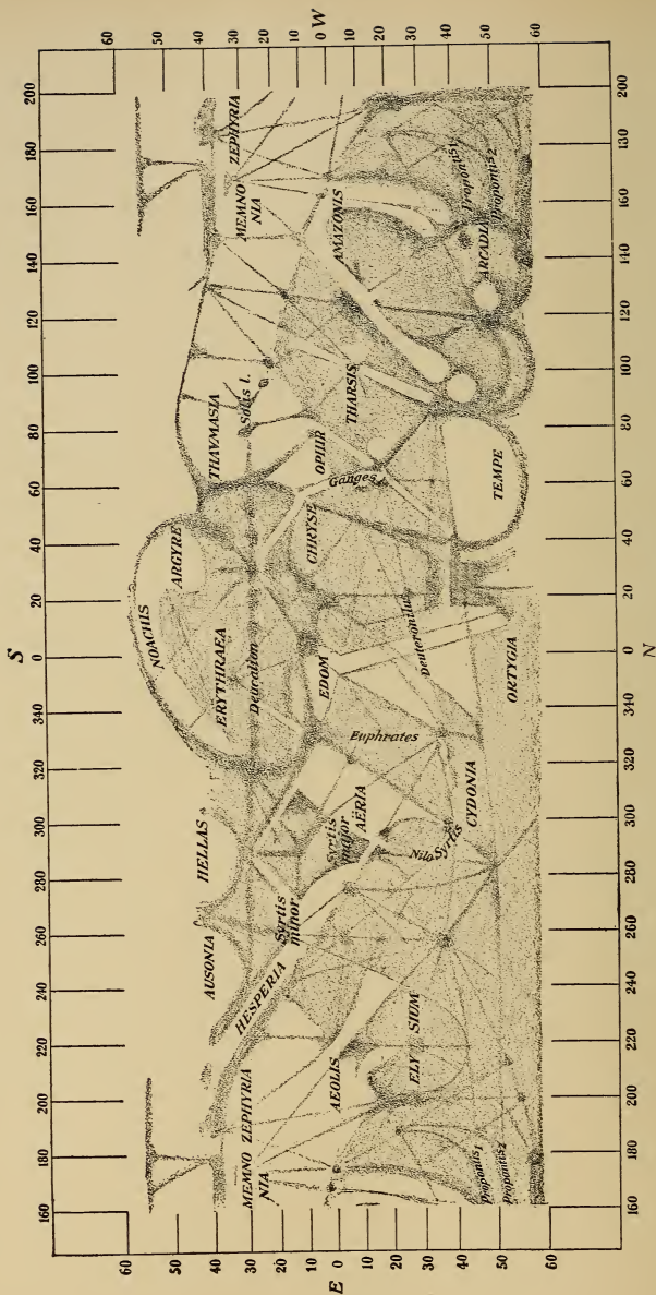
FIG. 43.—Chart of Mars.
