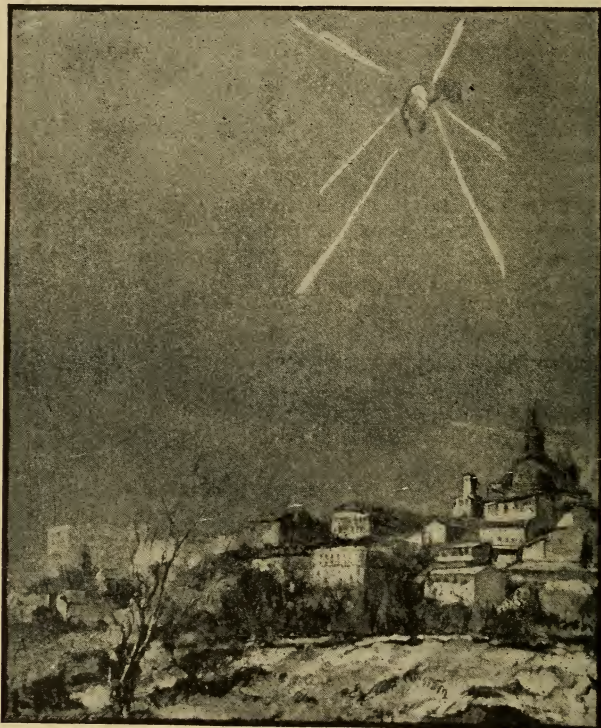
FIG. 57.—Explosion of a Fire-Ball above Madrid, February 10, 1896.
