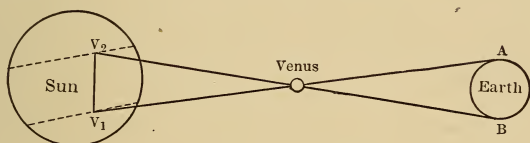
FIG. 83.—Measurement of the distance of the Sun.
