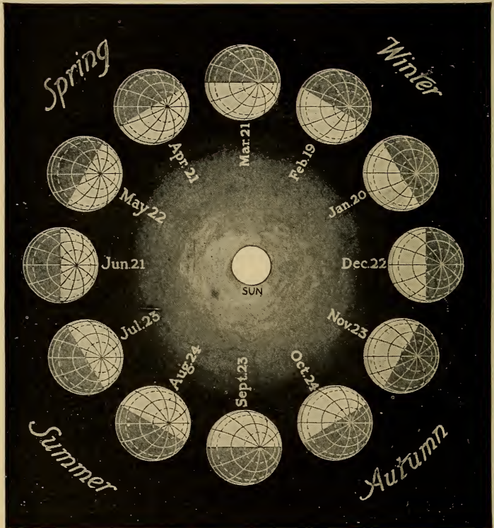
FIG. 60.—Motion of the Earth round the Sun.
