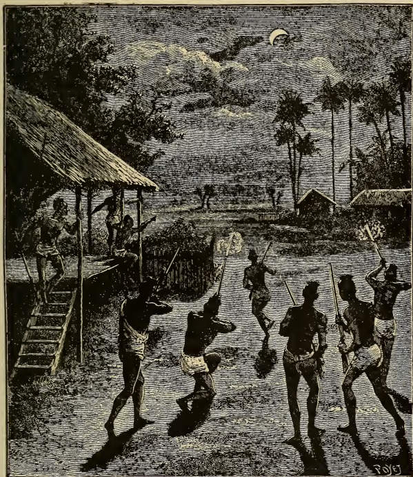
FIG. 76.—Eclipse of the Moon at Laos (February 27, 1877).
