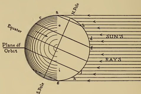
FIG. 61.—Inclination of the Earth.
