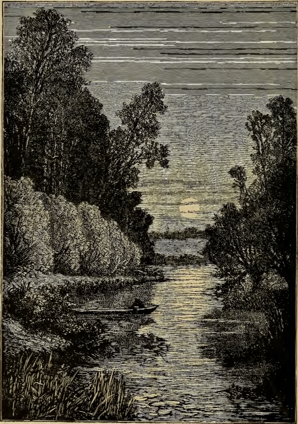
FIG. 64.—The Full Moon slowly rises.
