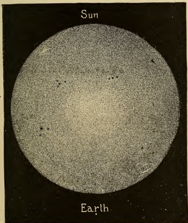
FIG. 28.—Comparative sizes of the Sun and Earth.
