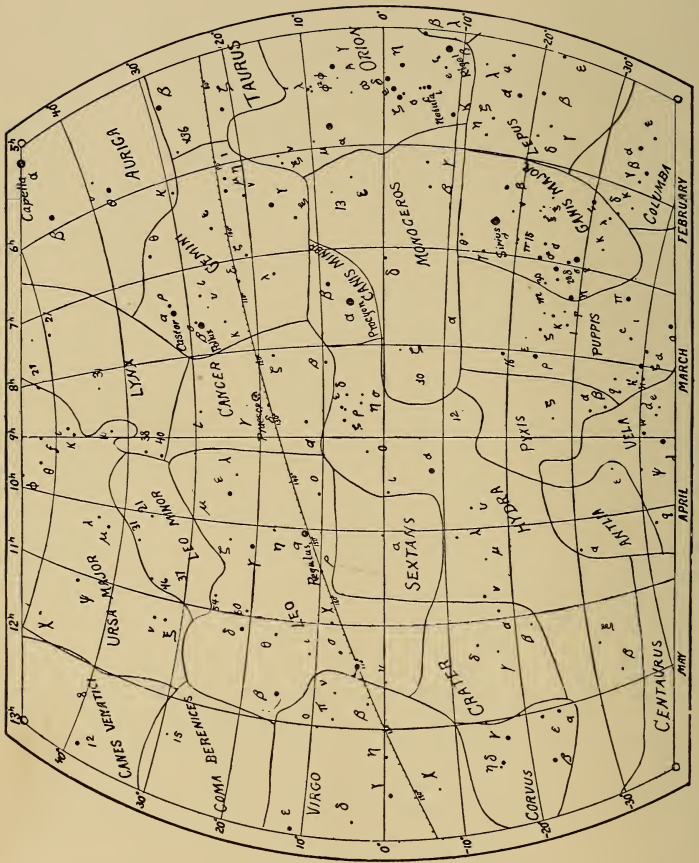
FIG. 14.—Spring Constellations.
