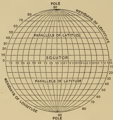
FIG. 62.—The divisions of the globe. Longitudes and latitudes.
