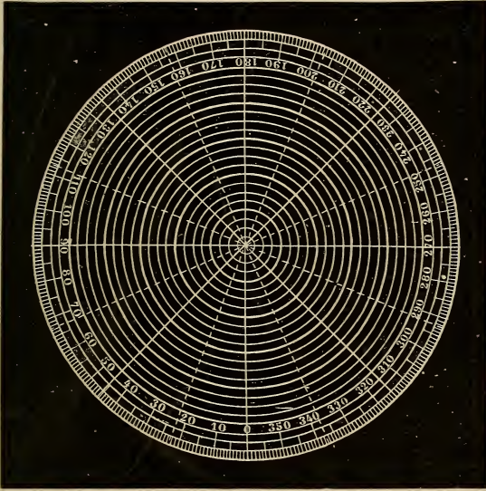
FIG. 81.—Division of the Circumference into 360 degrees.
