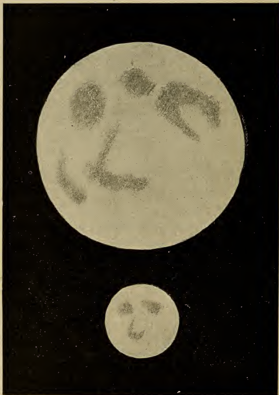
FIG. 65.—The Moon viewed with the unaided eye.
