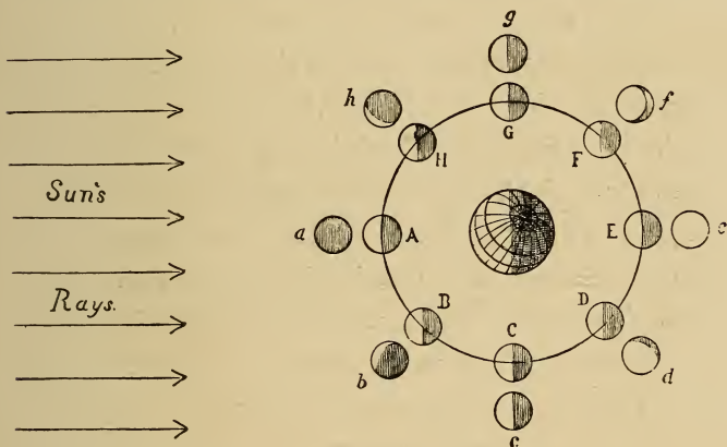
FIG. 70.—The Moon's Phases.
