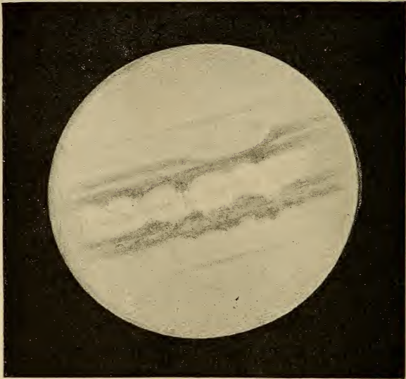
FIG. 45.—Telescopic aspect of Jupiter.
