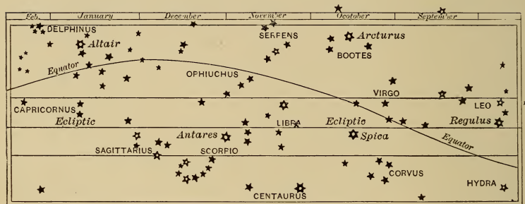
FIG. 10.—The Constellations of the Zodiac: summer and autumn; Capricorn, Archer, Scorpion, Balance, Virgin, Lion.
