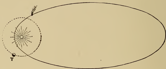
FIG. 52.—The orbit of a Periodic Comet.
