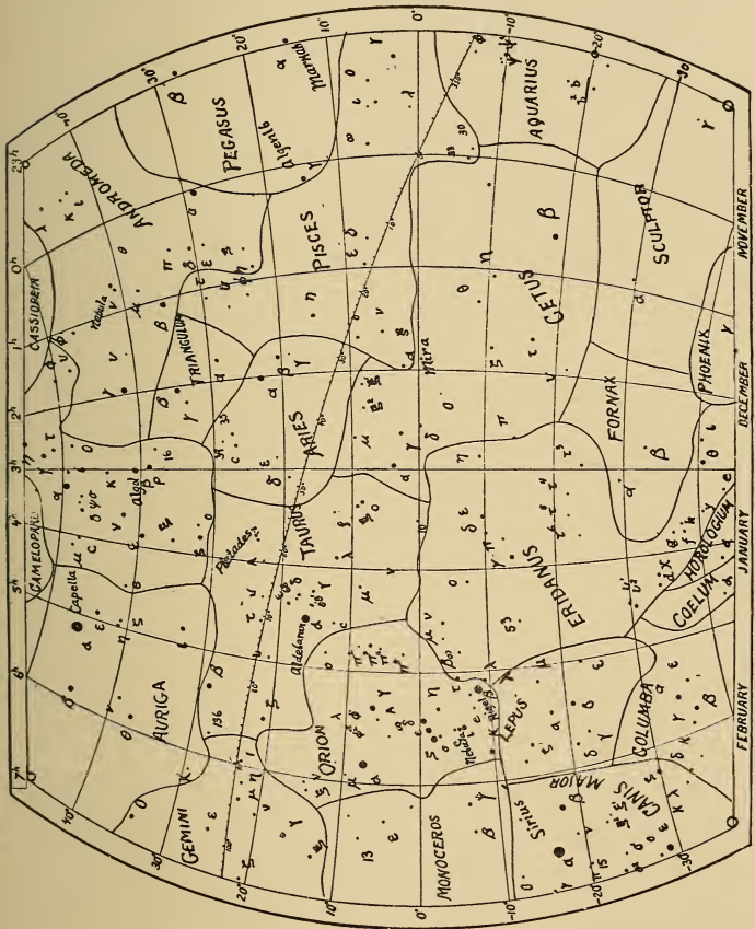
FIG. 13.—Winter Constellations.
