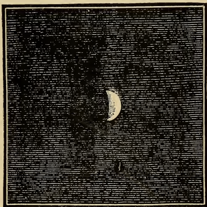
FIG. 34.—Mercury near quadrature.
