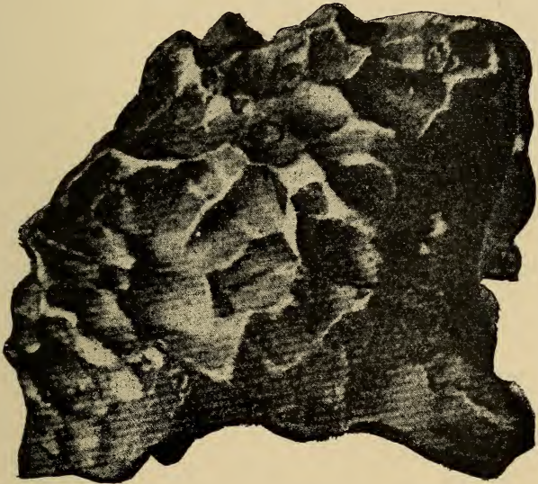
FIG. 59.—A Uranolith.
