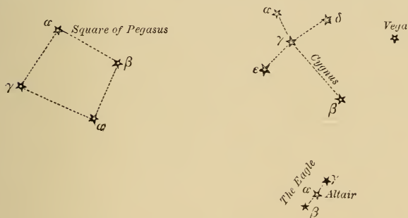
FIG. 9.—The Swan, Vega, the Eagle.
