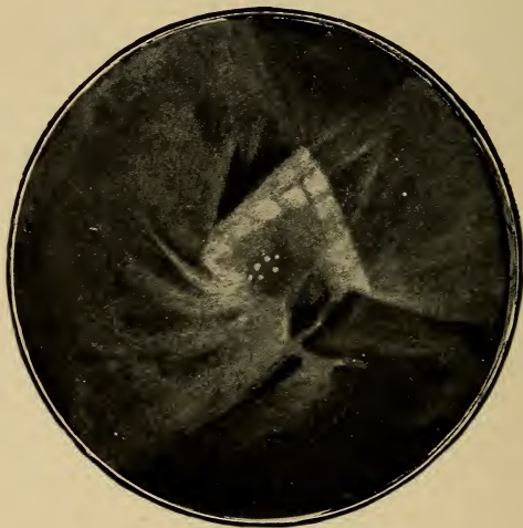
FIG. 20.—Sextuple star \theta in the Nebula of Orion.
