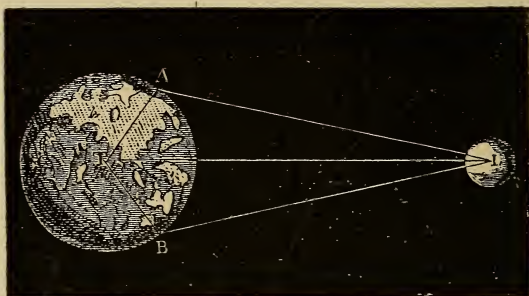
FIG. 82.—Measurement of the distance of the Moon.
