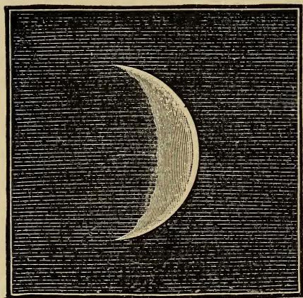
FIG. 38.—Venus at greatest brilliancy.
