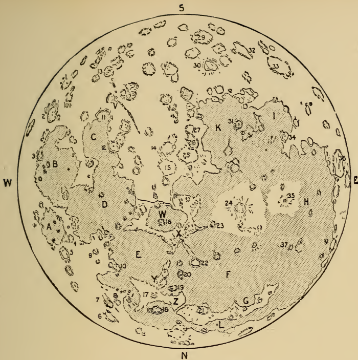
FIG. 71.—Map of the Moon.
