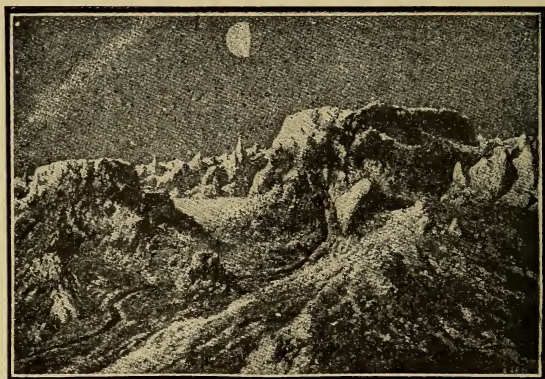
FIG. 74.—Lunar landscape with the Earth in the sky.
