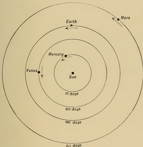
FIG. 32.—Orbits of the four Planets nearest to the Sun.
