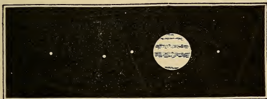
FIG. 46.—Jupiter and his four principal satellites.
