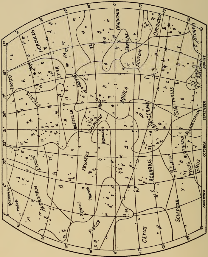
Fig. 16.—Autumn Constellations.
