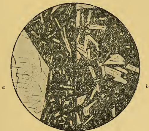
FIG. 1a.—Cumbraite, N.N.W. dyke, Eerie Port, Great Cumbræ. \times 20 . Large phenocryst of anorthite; groundmass: laths of labradorite, enstatite, augite, in base of dark glass. ,, 1b.—Cumbraite (Eskdalemuir type), W.N.W. dyke, Waterhead Burn, Muirkirk, Ayrshire. \times 20 . Microphenocrysts of labradorite and magnetite; groundmass: felspar microlites, grains of augite and enstatite, in base of dark glass.
