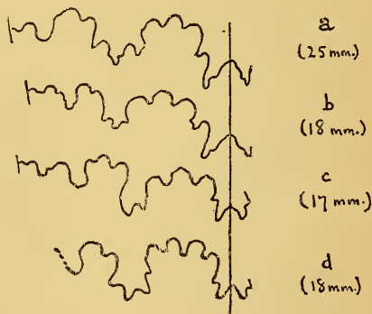
FIG. 12.—Adult sutures of Polymorphites . a, P. trivialis ; b-d, P. mixtus .
