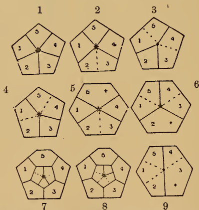
FIGS. 1-9.—Diagrams summarising the views of Wachsmuth & Springer on the structure of the Crinoid base. The posterior basal is numbered 5. The region where addition is supposed to have taken place is marked +.
