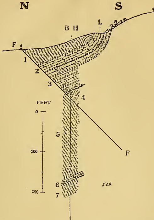
FIG. 2.—Vertical section, in a north and south plane, of the upper part of the Folly Farm Borehole, Presteign. L, lane; B H, borehole; F-F, overthrust fault; 1, 5, and 7, Wenlock Shales; 2, Woolhope Limestone and Shales; 3, Upper Llandovery Sandstone; 4, supposed Archæan (Longmyndian); 6, 12 ft. limestone-band.
