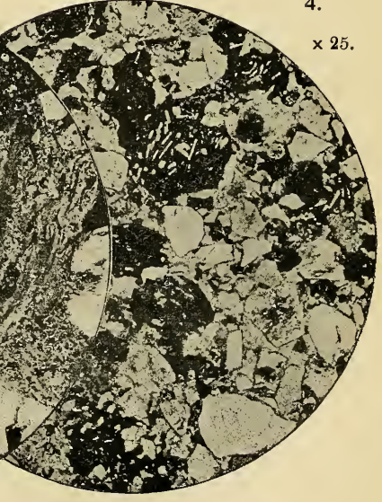
ROCK-SECTIONS, PAHANG VOLCANIC SERIES, F. M. STATES.
