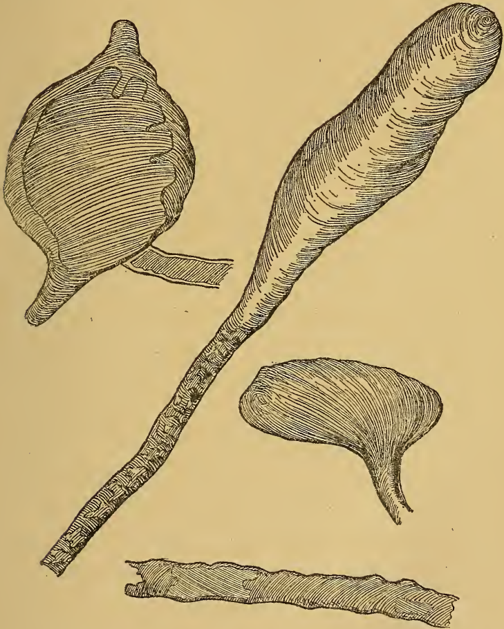
Sketch of animal remains in Dunliath Ferruginous Limestone (Jurassic), N.W. Scotland, found in association with fungal hyphæ. \times 1400 .
