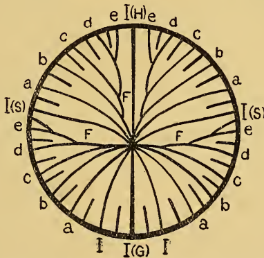
TEXT-FIG. 3. — Diagram of the calice of Hadrophyllum pauciradiatum , Edwards & Haime. H , G , S , Main, Counter, and Alar septa respectively. a-e , secondary septa. F , F' , F'' , Fossulæ. (After Duerden, 1905.) Nat. size.
