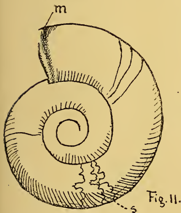
FIG. 11.— P. mixtus . s, last suture; m, mouth margin.
