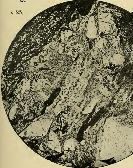
ROCK-SECTIONS, PAHANG VOLCANIC SERIES, F. M. STATES.
