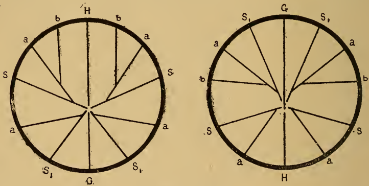
TEXT-FIG. 4.—Diagrammatic sections of Lophophyllum proliferum , McChesney. The section on the left is a Russian and on the right an American specimen. In both cases the upper side of the section is on the convex side of the polyparium (after Yakovlev & Duerden, 1903). H , G , S , Main , Counter , and Alar septa respectively. S 1 , the fourth pair of primary septa. a , b , secondary septa. \frac{2}{3} nat. size.
