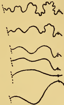
FIG. 13.—Sutural development of Cymbites globosus (after Branco).
