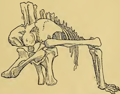
FIG. 2.—Posterior aspect of the pelvis and hind-limb of Diplodocus (after Tornier).
