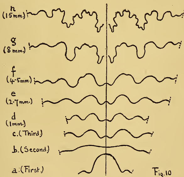
FIG. 10.—Sutural development, P. cf. jupiter .
