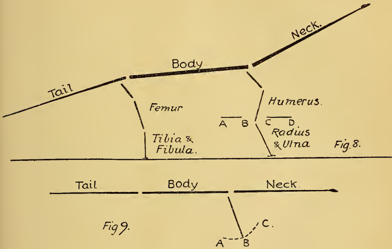
FIG. 8.—Diagram to illustrate wrong articulation of the limb-bones of the Diplodocus skeleton. The body, neck, and tail are shortened for convenience.
