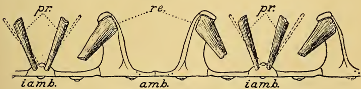
FIG. 5.—Schematic restoration of the attachment of the lantern muscles to the perignathic girdle in Plesiechinus . pr. protractors, re. retractors. The hypothetical radial compass muscles are indicated by double broken lines.
