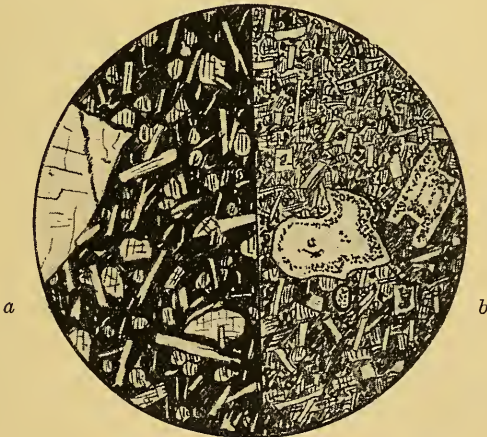
FIG. 2a.—Tholeiite (Brunton type), N.N.W. dyke, Stairaird, River Ayr, near Mauchline, Ayrshire. \times 20 . Large phenocryst of bytownite-anorthite; groundmass: grains of augite, and laths of labradorite, in base of dark glass.
