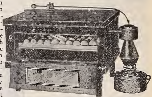
Buckeye Style A 60-Egg Incubator
