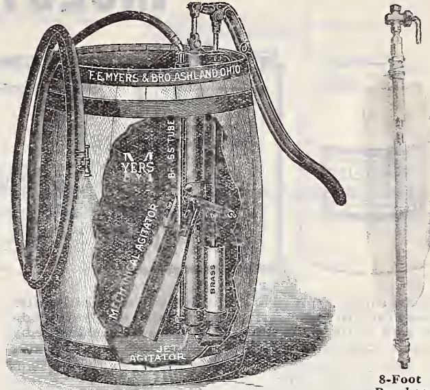
Myers' Improved Orchard Barrel Spray Pump No. 305
