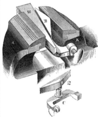
Improved Vise Attachment.
