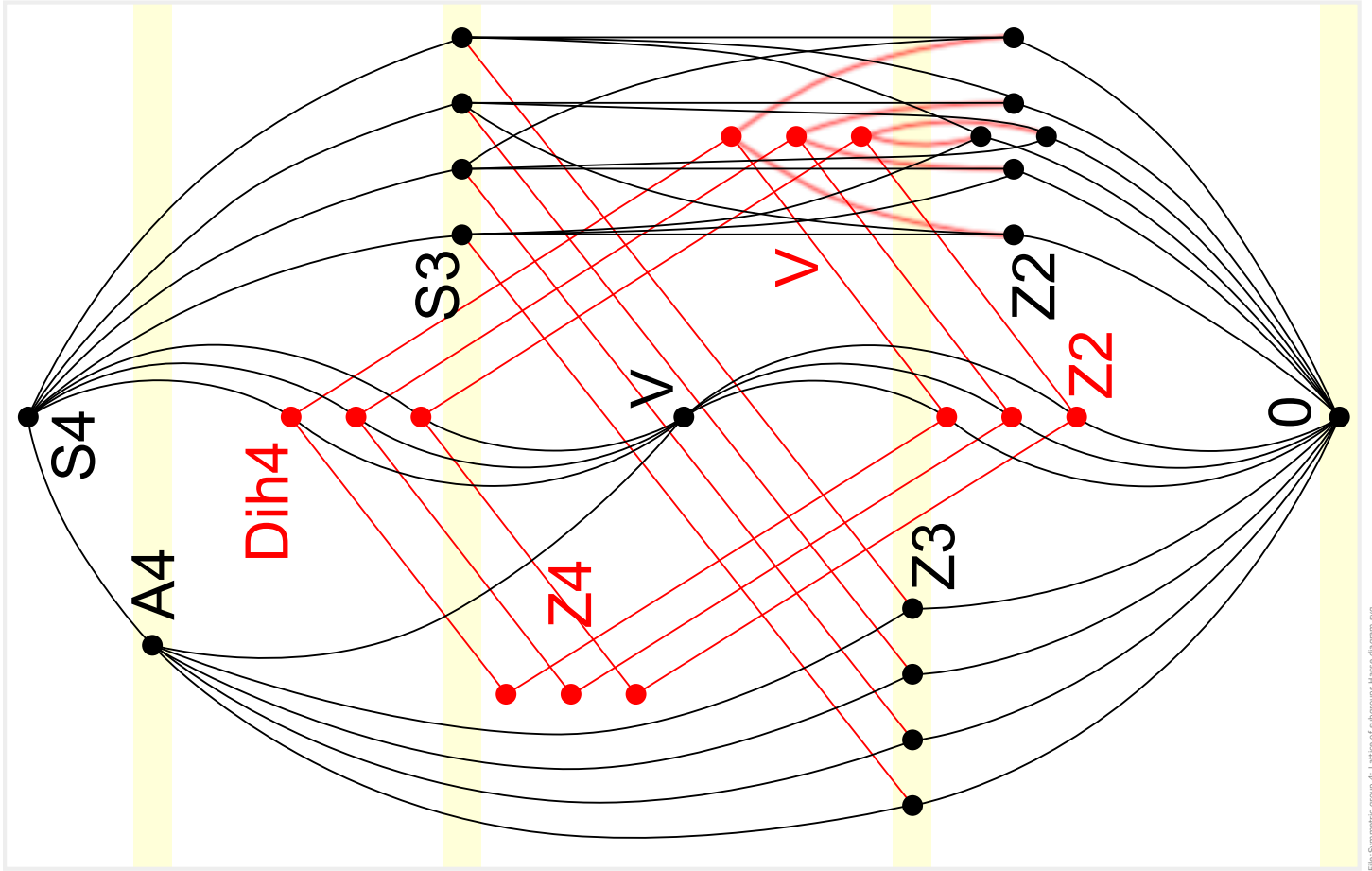
File:Symmetric_group_4_Lattice_of_subgroups_Hasse_diagram.svg
