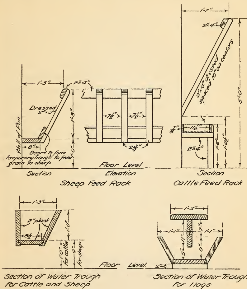
FIG. 6.—Details of equipment for yard shown in figure 3.
