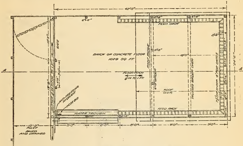
FIG. 3.—Plan of single yard for unloading stock.
