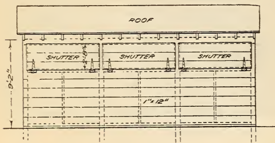
FIG. 5.—End view of covered section of yard, showing doors to be dropped for ventilation.
