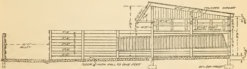
FIG. 4.—Side view of yard shown in figure 3.
