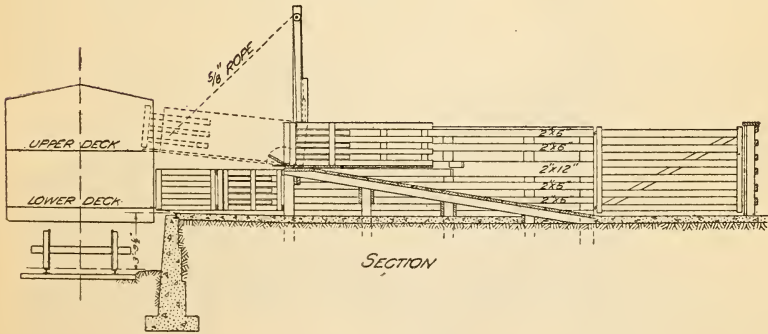
FIG. 1.—A good arrangement for unloading double-deck cars.
