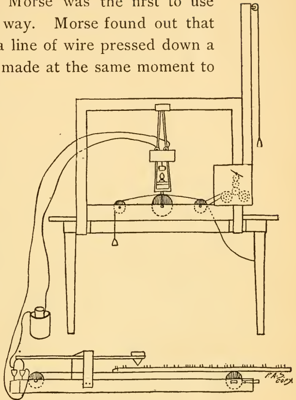
THE FIRST MORSE INSTRUMENT.
