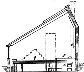
FIG. 3. MODEL GREENHOUSE OF 1835.
