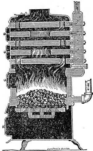
FIG. 68. SPENCE HEATER.
