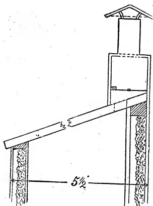
FIG. 112. A CHEAP HOUSE (Section).
