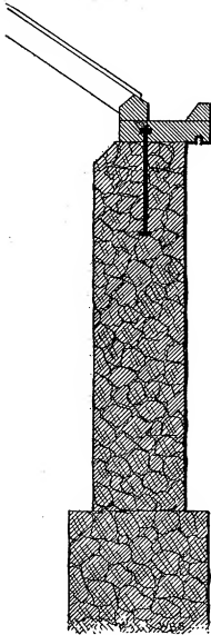
FIG. 11. GROUT WALL.
