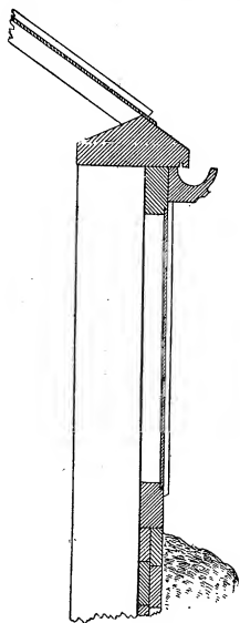
FIG. 16. WOODEN WALL WITH GLASS SIDE.
