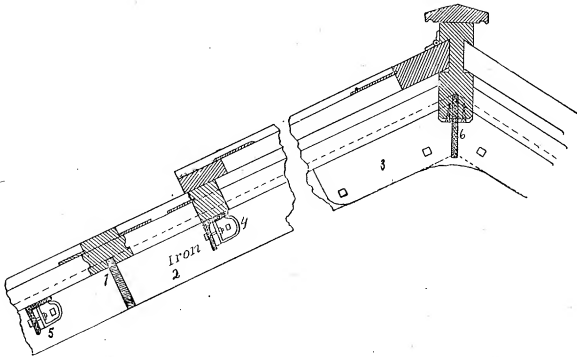
FIG. 26. DETAILS FOR COMBINED IRON AND WOOD ROOF.
