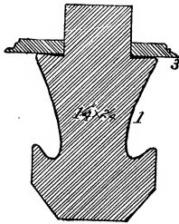
FIG. 18. SASH BAR WITH DRIP GUTTERS (Section).
