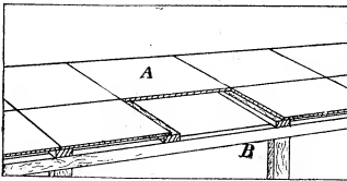
FIG. 56. WOOD AND SLATE BENCH.
