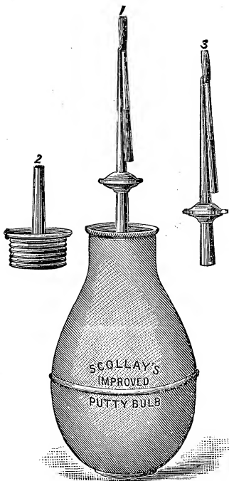
FIG. 38. PAINT BULB.
