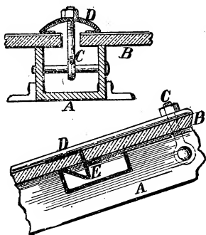
FIG. 32. PARADIGM GLAZING.
