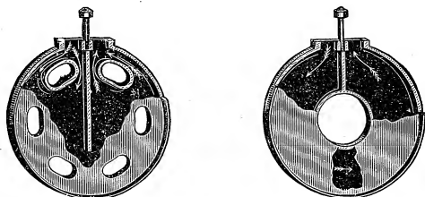
FIG. 69. SPENCE HEATER. FIG. 70. SPENCE HEATER. (1st, 3d and 5th Sections.) (2d and 4th Sections.)
