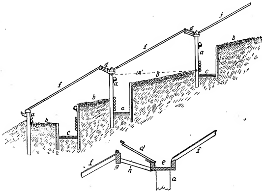
FIG. 8. SIDEHILL HOUSES ( Section ).
