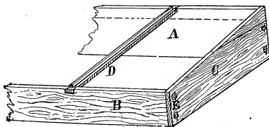
FIG. 84. HOTBED FRAME.
