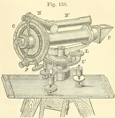
Dabbadie's Theodolite.
