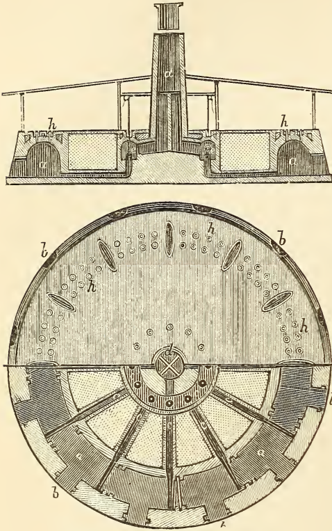
Hoffman's Annular Brick Furnace.
