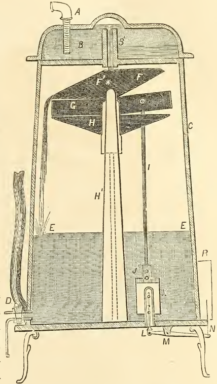
Cochrane's Water Meter—section.
