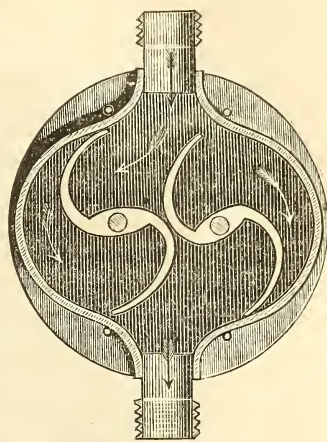
Payton's Meter for Liquids.
