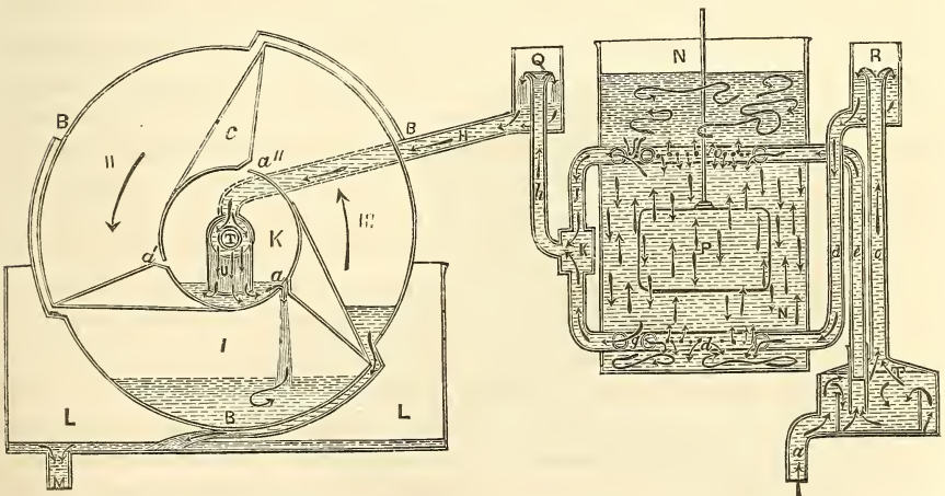
Siemens and Halske's Volumeter.
