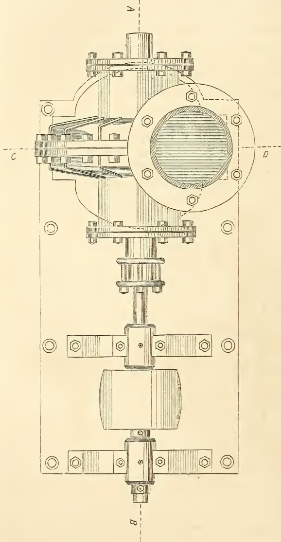
Gwynne &amp; Co.'s Centrifugal Pump—scale, 1-12.
