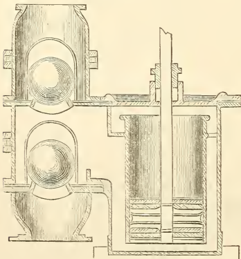
Schabaver and Foures's Pompe Castraise.
