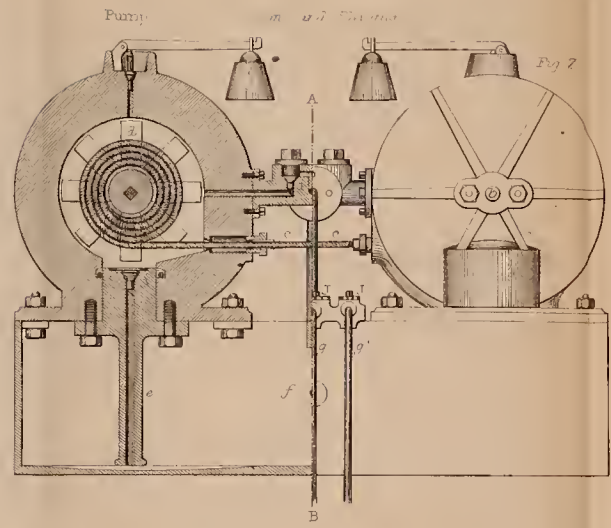
APPARATUS OF DESGOFRE AND OLLIVIER
