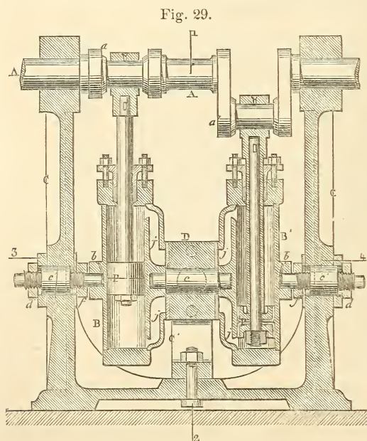
Ramsbottom's Water-engine.
