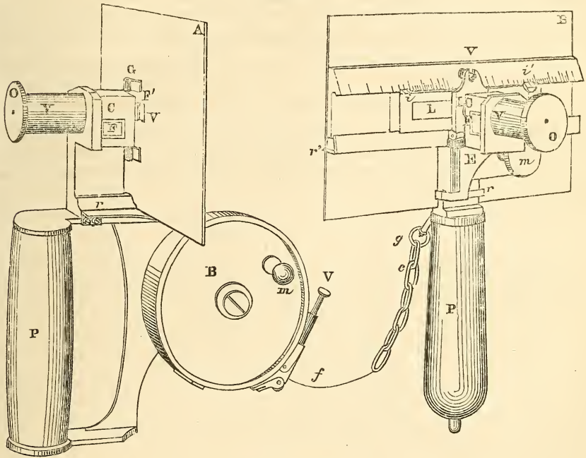
Prism Telemeter.
