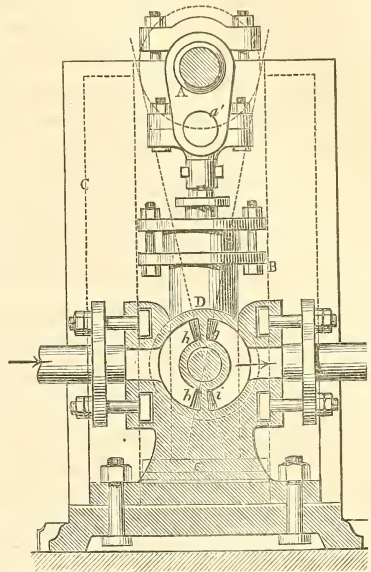
Ramsbottom's Water-engine.
