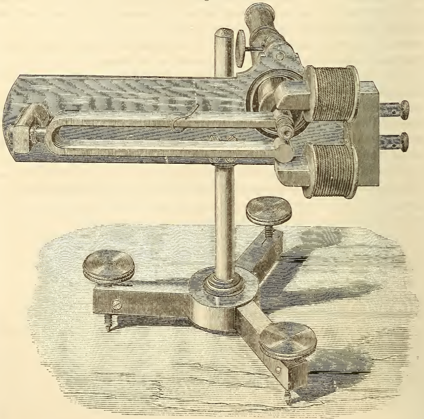
Lissajous's Comparator.
