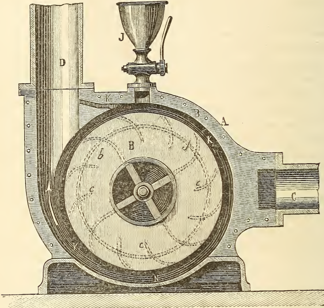
Neut & Dumont's Centrifugal Pump—vertical section.
