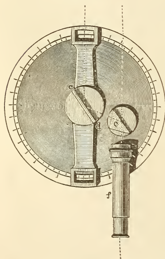
Pistor &amp; Martens's Circle.
