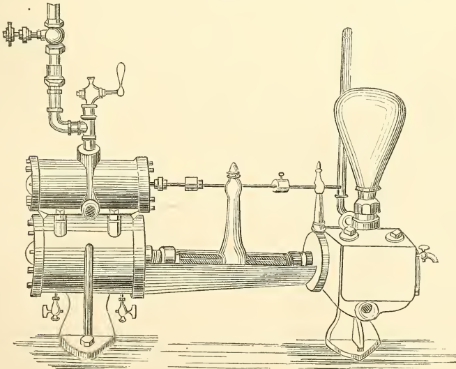
Earle's Steam-pump.
