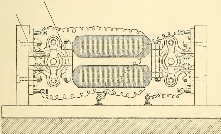
Ladd's Dynamo-electric Machine—elevation.
