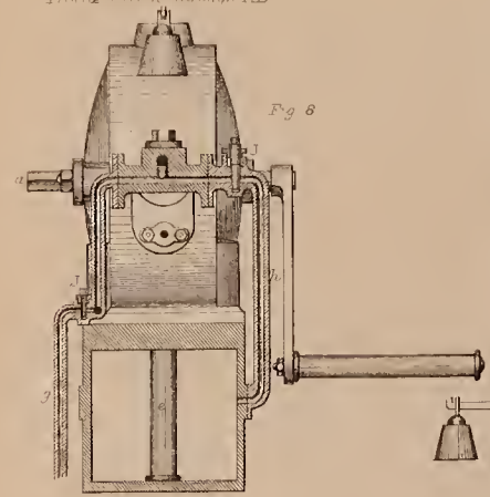
APPARATUS OF DESGOFRE AND OLLIVIER
