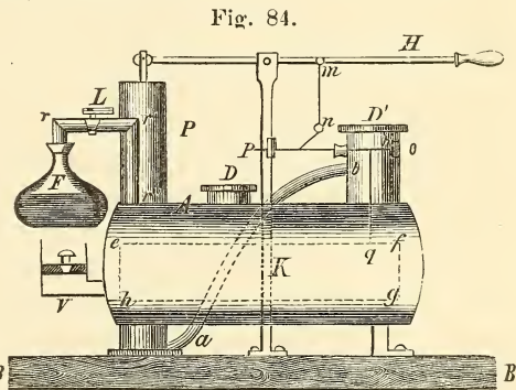
Carré's Sulphuric Acid Freezing Apparatus.
