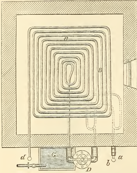
Marval's Heating Apparatus—plan.
