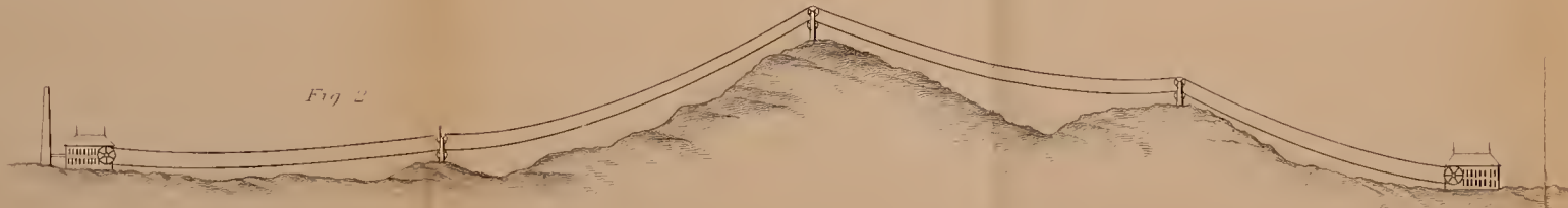
A telodynamic cable passing a mountain
