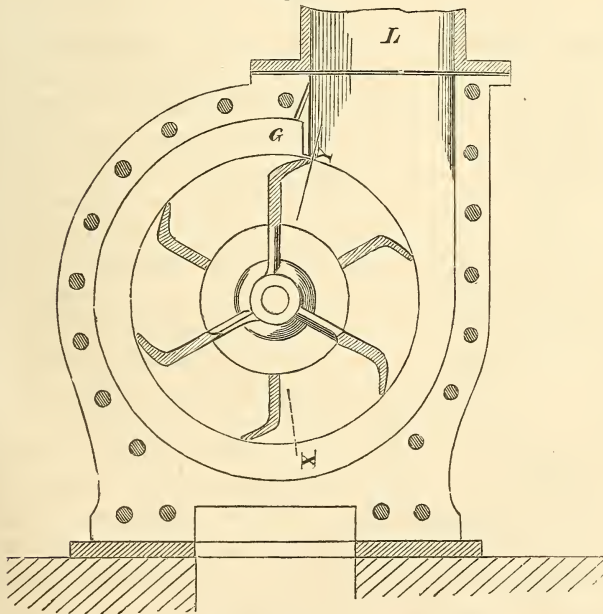
Gwynne & Co.'s Centrifugal Pump—scale, 1-12.
