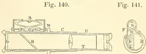
Davidson's Spirit-level Sextant.
