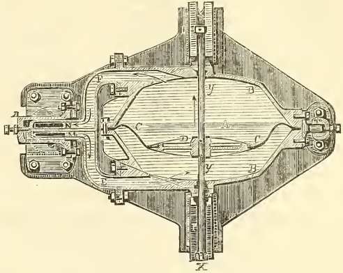
Duboys's Water Meter—interior.
