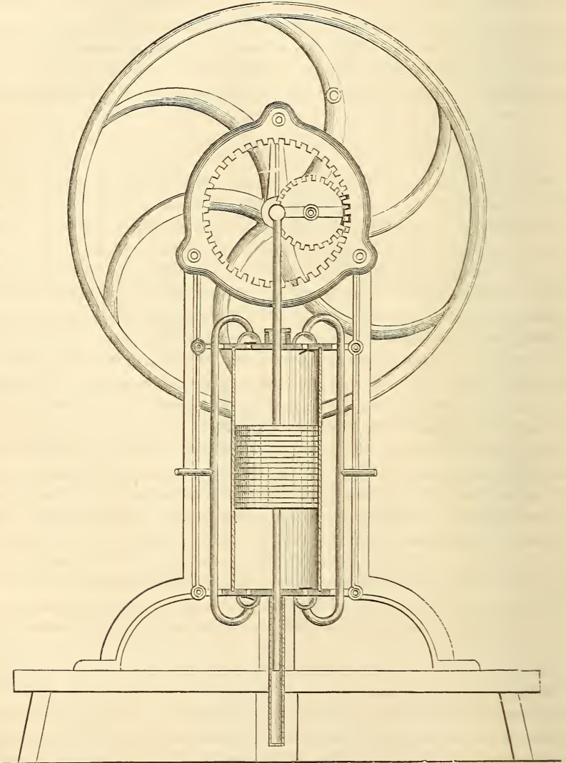
Deleuil's Free-piston Air-pump.
