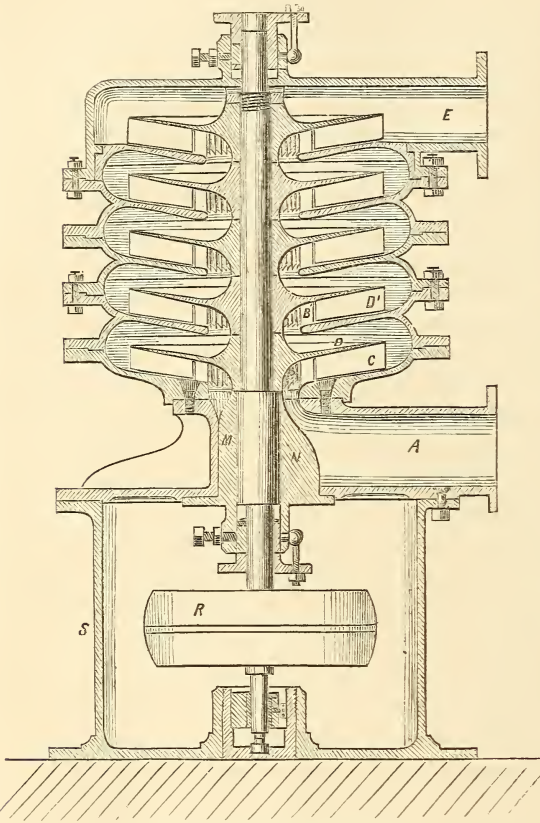
Girard's Turbine Elevator.
