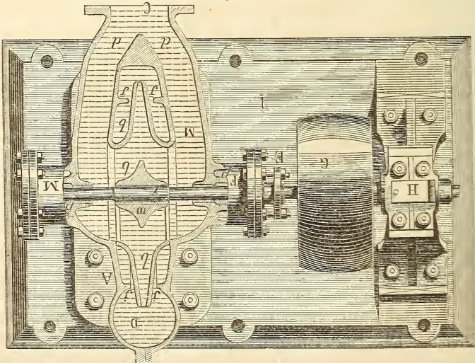
Neut & Dumont's Centrifugal Pump—horizontal section.
