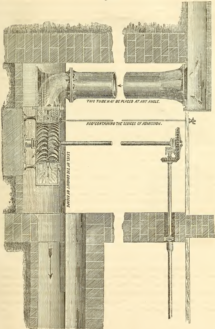
Schiele's Turbine.
