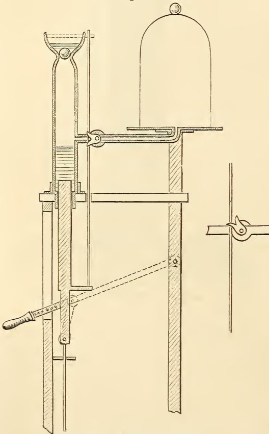
Kravogl's Mercurial Air-pump.
