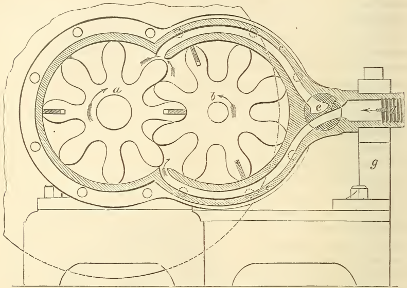
Pillner &amp; Hill's Rotary Engine.
