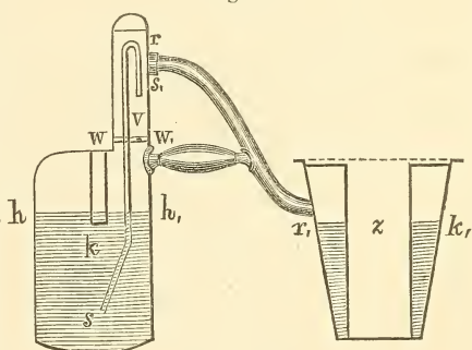
Carré's Ammoniacal Freezing Apparatus for families
