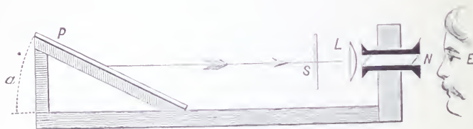
FIG. 11.—Simple Polarizing Apparatus.
