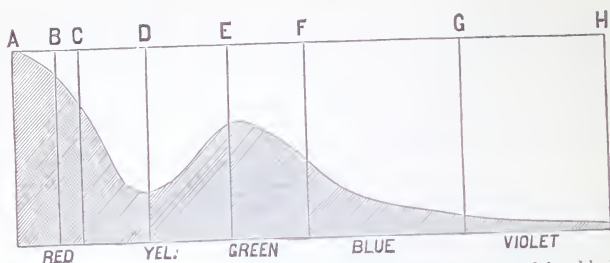
FIG. 21.—The shaded portion represents the amount of light transmitted by chloride of chromium.
