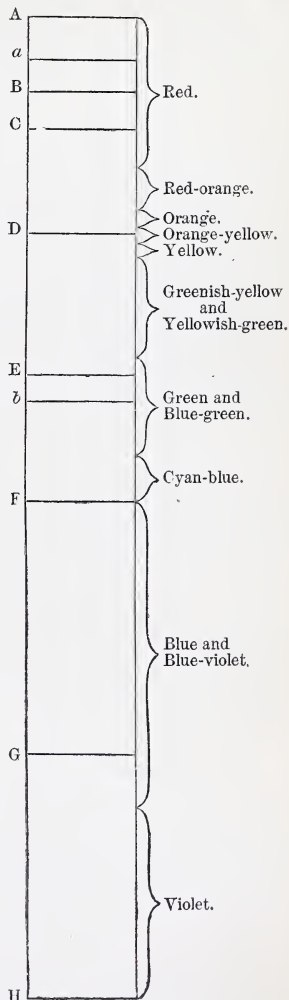
FIG. 46.—Prismatic Spectrum.
