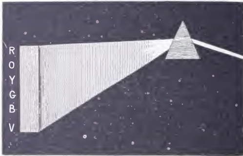
FIG. 1.—Prismatic Spectrum.
