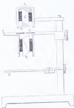
FIG. 63.—The Schistoscope, for the production of Complementary Colours. (Brücke)
