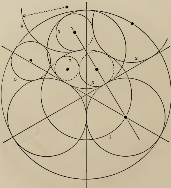
The curves Nos. 1 and 4 are of similar radius.
