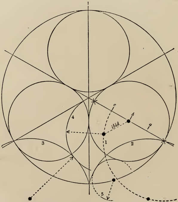
The arcs 1. 2. 3. are of the same radius.
