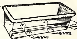
Diagram shows the interior construction of the S. & W. Co.'s Irrigating Flower-Box
