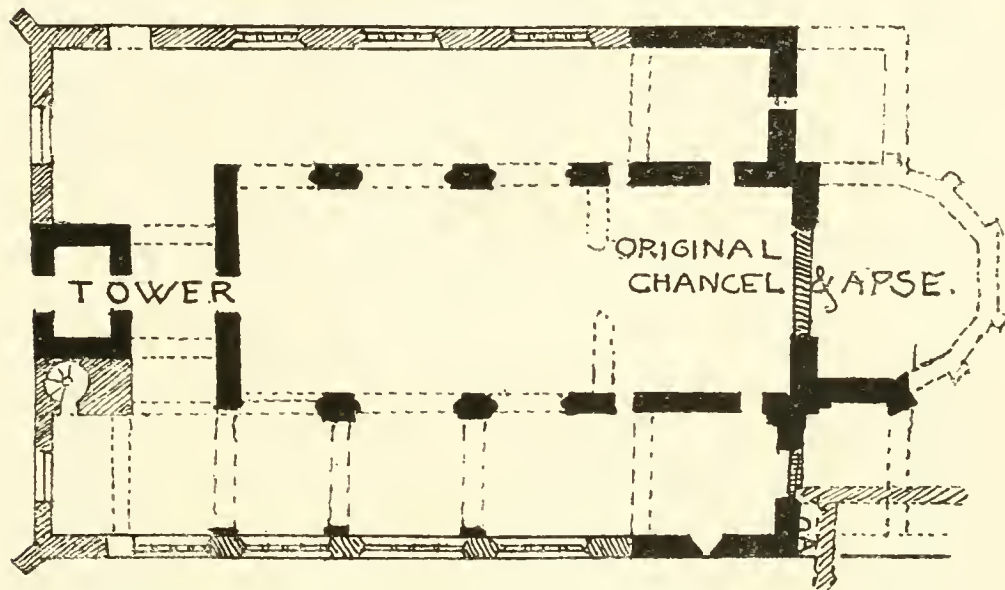
DEERHURST, CH. (after Butterworth.) Feet. 0 5 10 20 30 40 50 60 70 80 90
