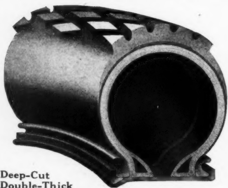
The New Goodyear Non-Skid Tread
