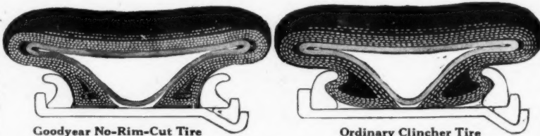
Goodyear No-Rim-Cut Tire
