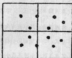
(c) r = 0
