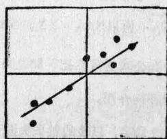
(b) r > 0 < 0
