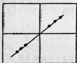
(a) r = 1
