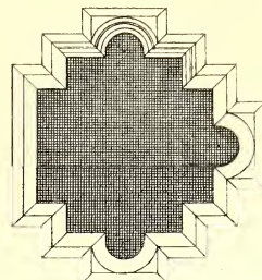
Column in Nave. 1/4 inch to a foot.
