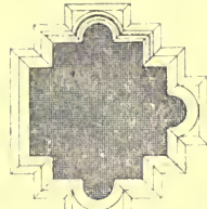
Column in Nave. 17 inch to a foot.
