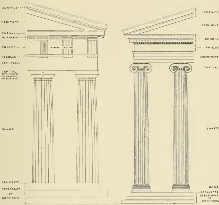
THE DORIC AND IONIC ORDERS COMPARED
