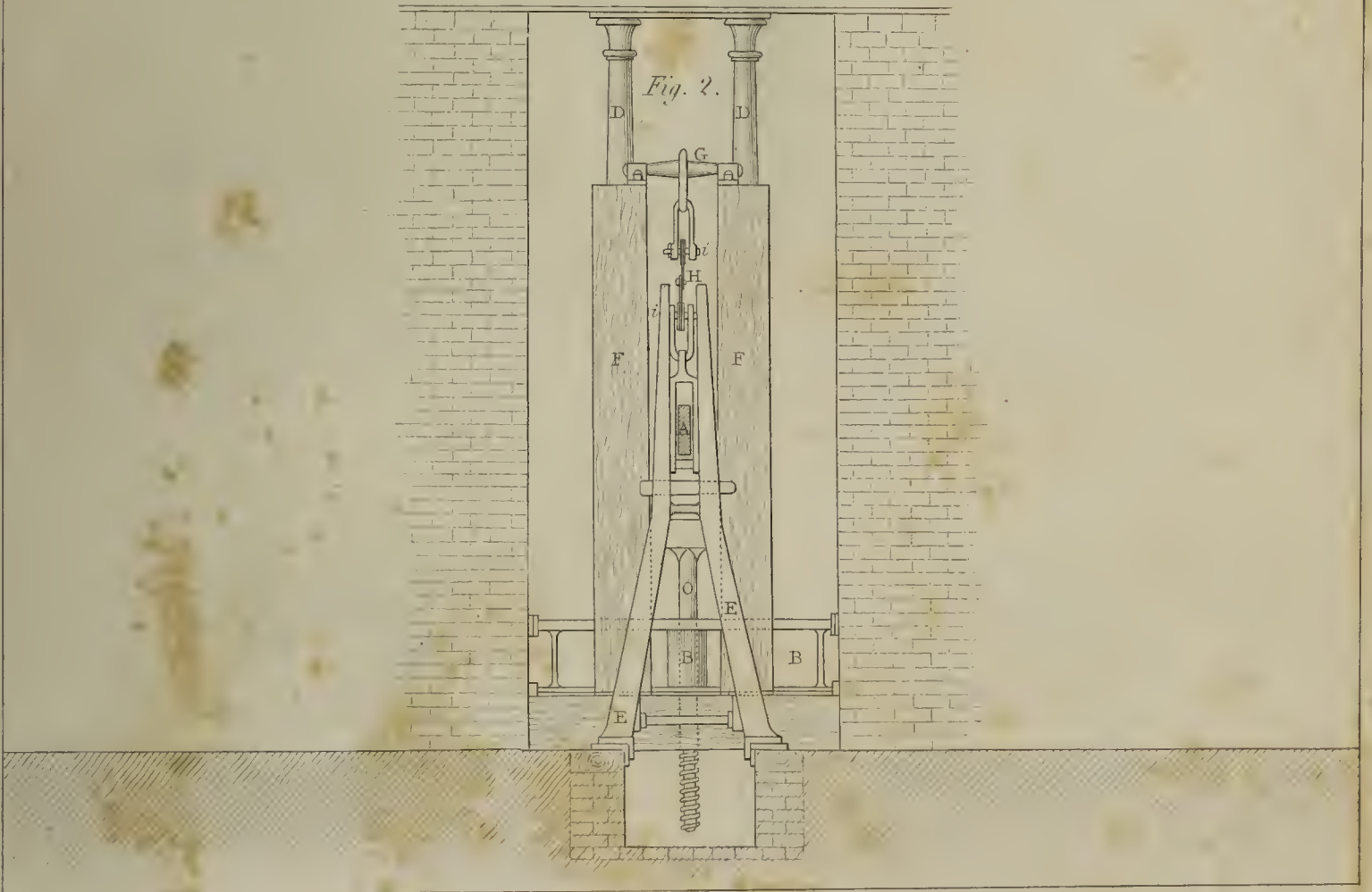
End View.
