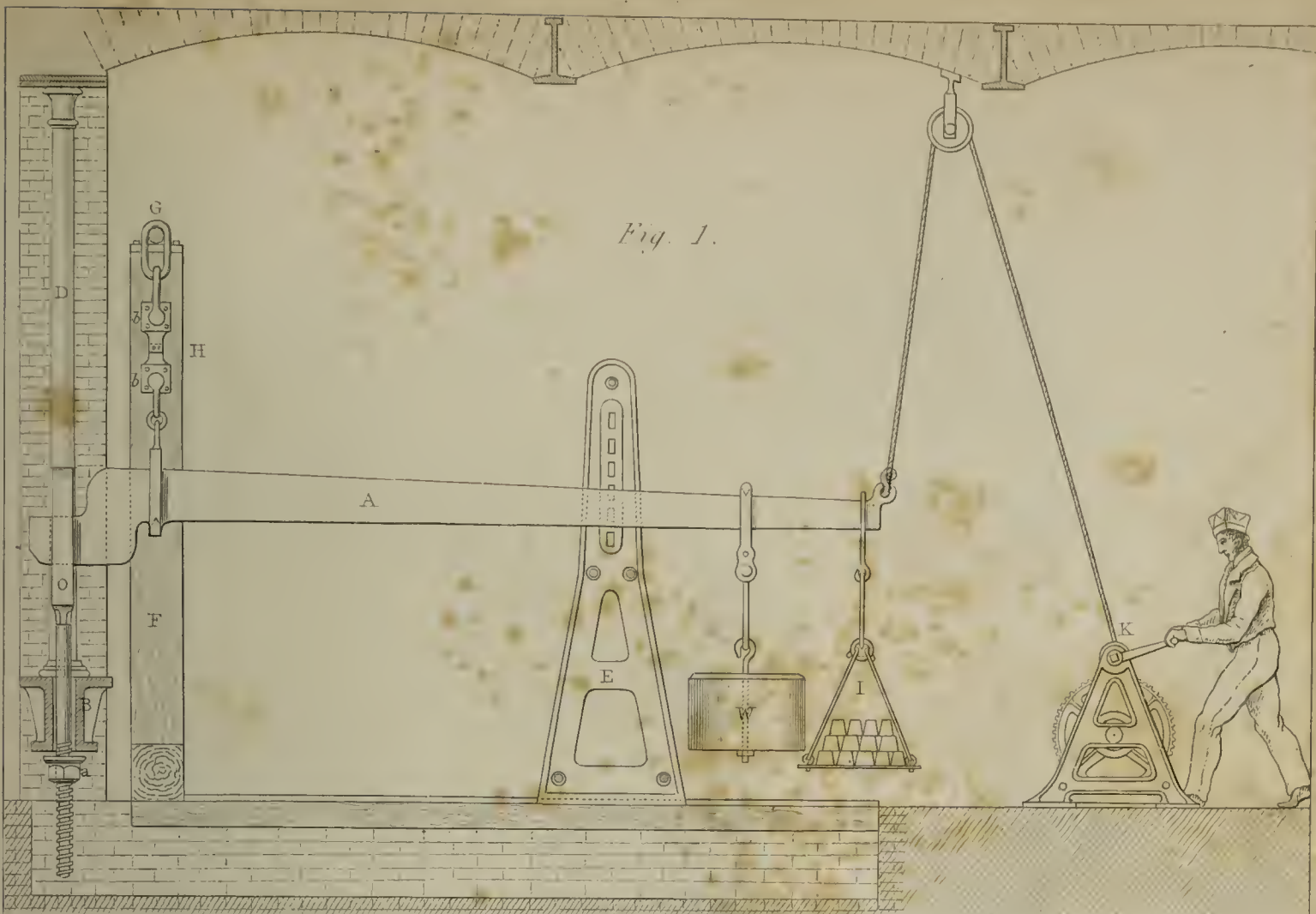
Side View.
