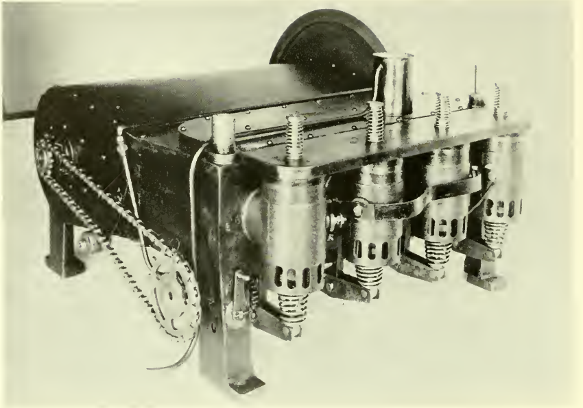
1. Wright brothers' engine from 1903 airplane.
