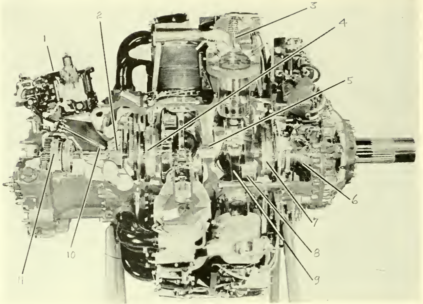
1. Pratt & Whitney R-2800, 18-cyl., 1946 (cutaway). 1, Injection carburetor; 2, supercharger rotor; 3, inlet valve; 4, rear cam drum; 5, center main bearing; 6, planetary reduction gear; 7, front cam drum; 8, front counterweight; 9, front master rod; 10, fuel nozzle; 11, supercharger drive gears.
