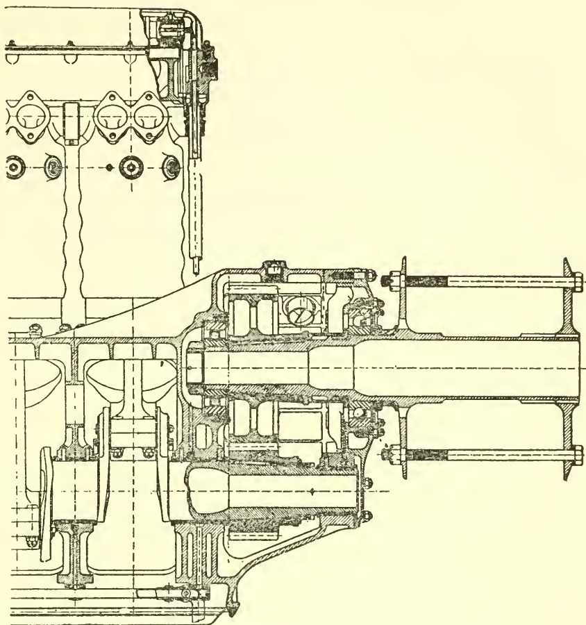
FIGURE 17.—Reduction gears of Renault Type 12 Kh engine.
