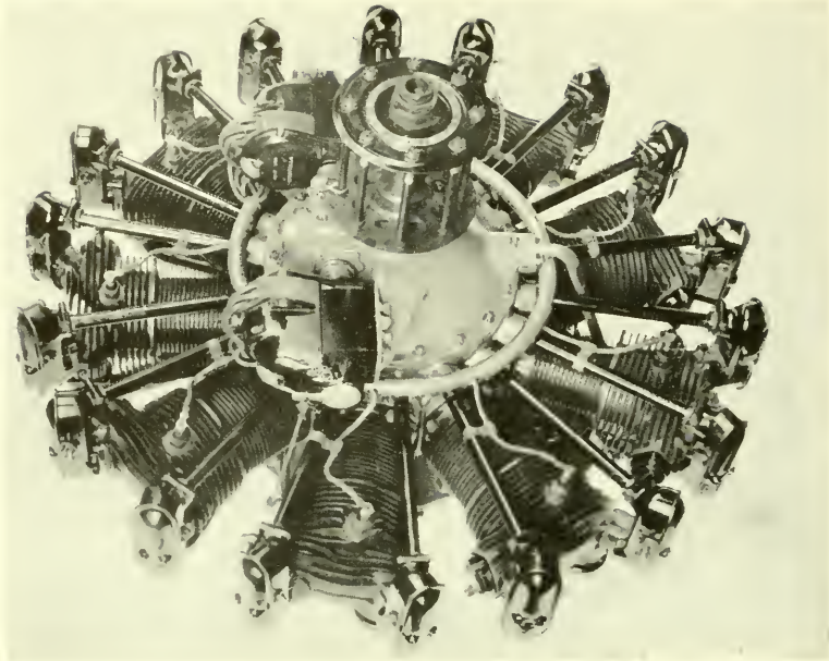
2. Wright Whirlwind engine of 1927. This type of engine was used by Lindbergh, Chamberlin, Byrd, and others.
