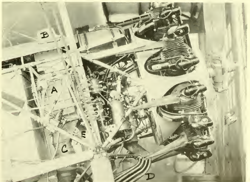
2. N.A.C.A. Roots type supercharger, coupled to Pratt & Whitney "Wasp" engine in a Wright Aero Corp. "Apache" airplane. This installation broke the world altitude record in 1927. This was the only successful displacement-type supercharger. A, Supercharger; B, air intake; C, delivery pipe through intercooler D; E, supercharger bypass.
