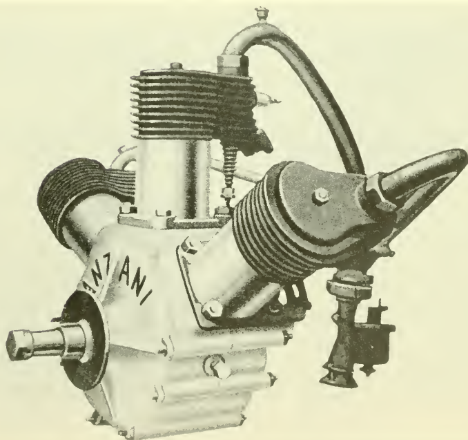
2. Anzani 3-cylinder fan-type engine, 22 hp., 1909.
