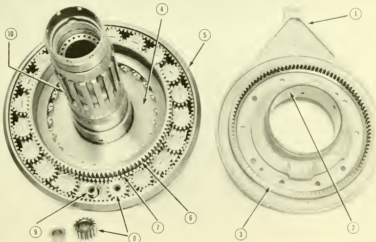
2. Modern planetary spur gear as used on radial engines. (Courtesy Wright Aeronautical Corp.) 1, Torque-meter arm; 2, bearing on propeller shaft; 3, spline for holding sun gear stationary; 4, propeller-shaft disc carrying pinions; 5, ring gear attached to crankshaft; 6, sun-gear spline; 7, sun gear (stationary); 8, pinions; 9, pinion shaft; 10, propeller shaft.
