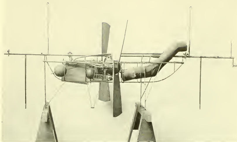
1. Langley steam engine used in Aerodrome No. 5, 1896.
