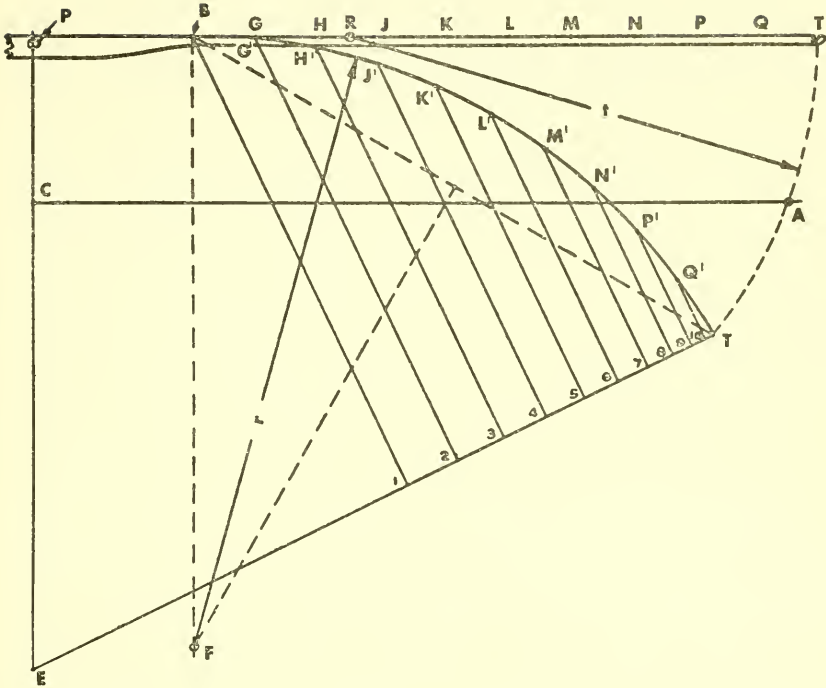
FIGURE 6.—Graphic method of designing a bow. BT , the limb, is divided into ten equal sections. Its tip, in bending, follows the path TT' , a circular arc with center at R and radius t , which is 3/4 BT in length. The length of the arrow is EP ; the line CA represents the string on the braced bow, with CP the "bracing height"; ET' represents the string at full draw. Arc BT' represents the bent limb, with radius r , the center of which is located by the intersection of the line BF which is perpendicular to BT , and the perpendicular bisector of chord BT' . Perpendiculars to ET' are dropped from each of the ten equally spaced points B, G, H, \dots, Q , along the bent limb. The lengths of the perpendiculars are proportional to the respective widths of the limb at each of the ten locations.
