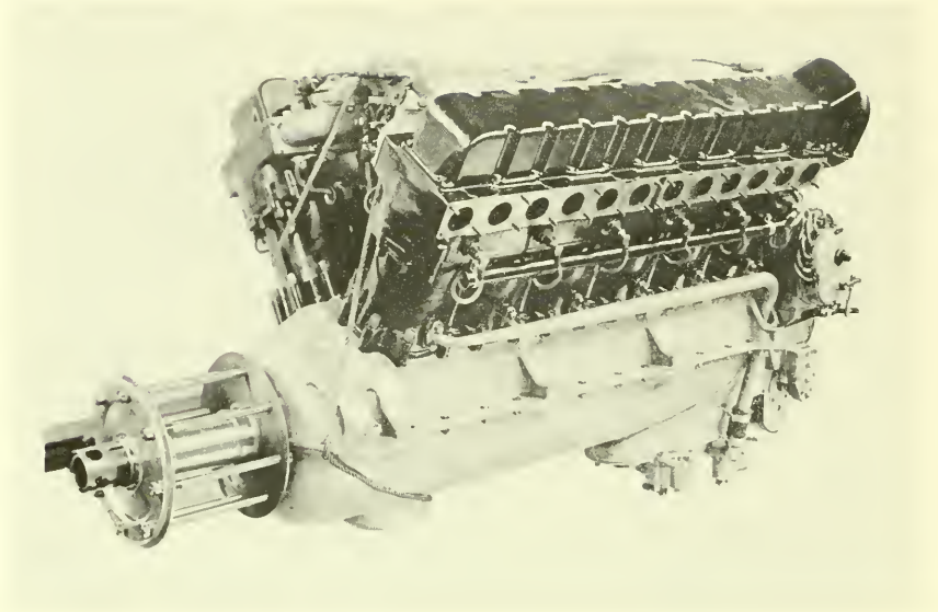
1. Curtiss D-12 engine, first to fly more than 200 m.p.h., Detroit, 1922.
