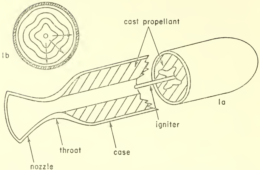
FIGURE 1.— a , Typical modern solid propellant rocket; b , recession of internal surface with time.
