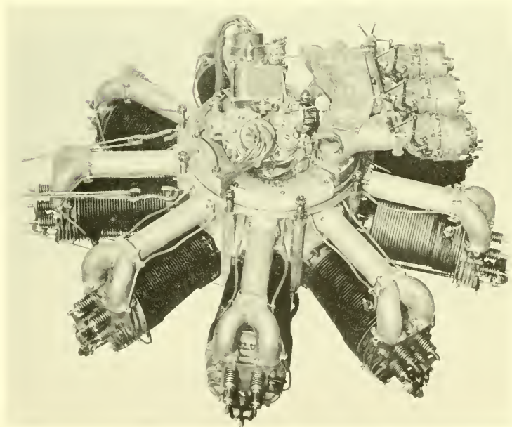
1. Bristol Jupiter, 1922, 360 hp., at 1600 r.p.m. This example was built by Cosmos Engineering Co., Ltd. (Photo from McCook Field Report 2193.)
