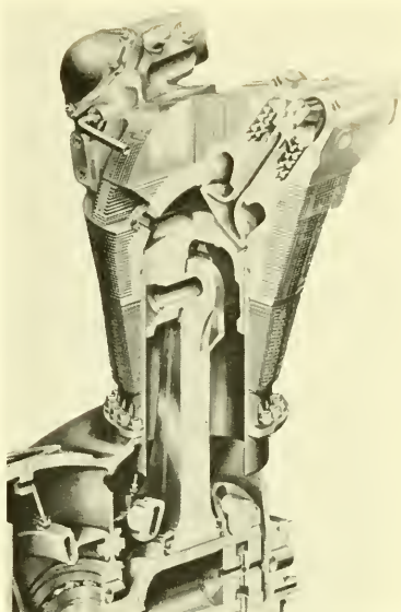
1. Forged cylinder for Wright 3350 engine, 1948. Forged and machined head, steel barrel with aluminum fins rolled in, sodium-cooled valves Stellite-faced, 100-plus square inches of fin area per square inch of piston area. (Courtesy Wright Aeronautical Corp.)
