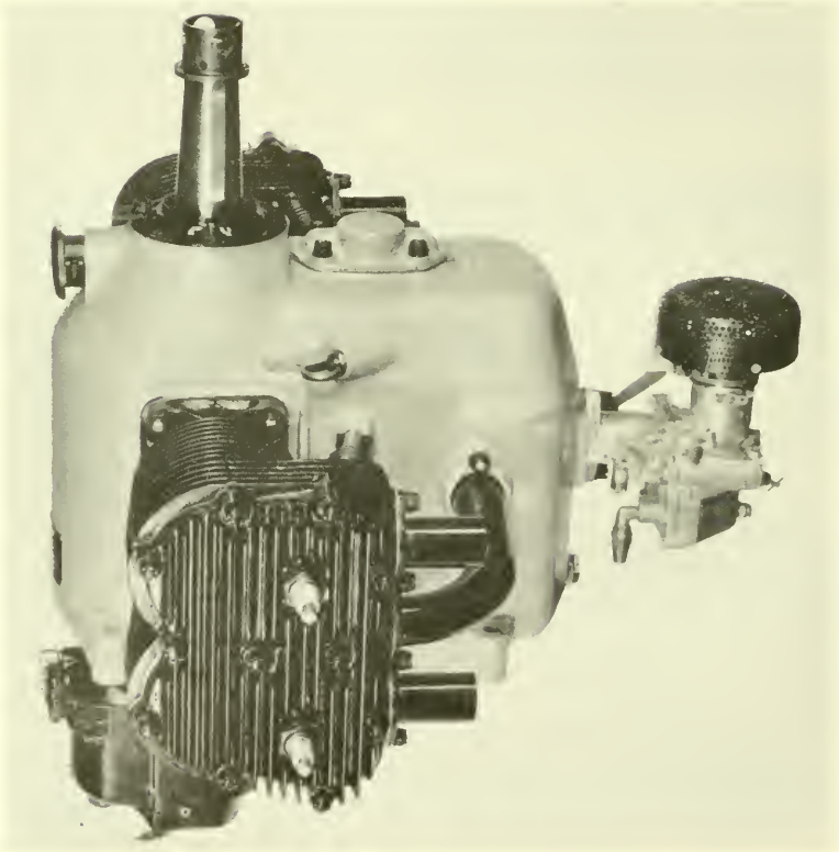
1. Continental A-40, 4-cyl. horizontal opposed, 38 hp., 1931.
