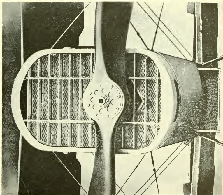
1. Large frontal coolant radiator for Liberty engine on DeH-4 airplane, 1918.
