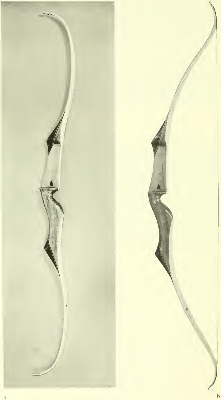
a b A modern composite bow (bow of the 1960's) (a) relaxed, (b) braced, and pl. 5, at full draw. Note the length (ca. 20") of the equal limbs, as compared with the 34" length of the upper and 32" lower limb of the English longbow of figure 1, and the rigid midsection, 27" long, which is completely absent in the English longbow. (Photos courtesy of Bear Archery Co.)
