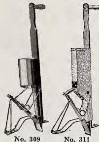
No. 311—Acme Segment Corn Planter
