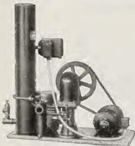
Ball-Bearing Pump
