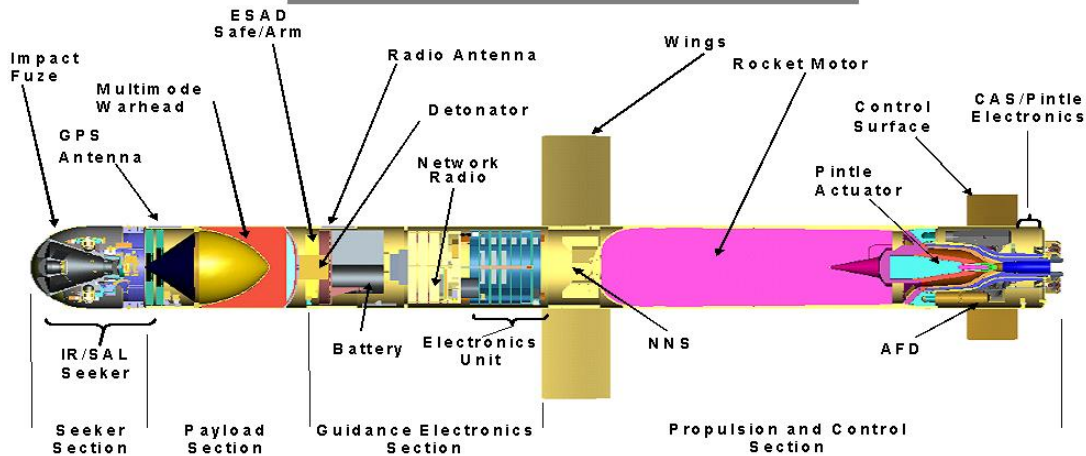
Figure 3: Precision Attack Missile (PAM) 8 . The PAM consists of a variable thrust motor, dual-mode precision uncooled infrared/semi-active laser seeker and a large multimode warhead effective against both moving and stationary targets.
