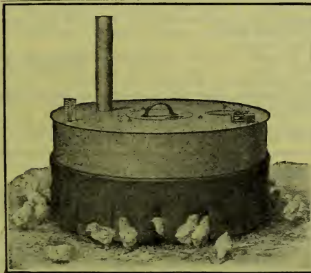
Cyphers New 1913 Portable Hover.
