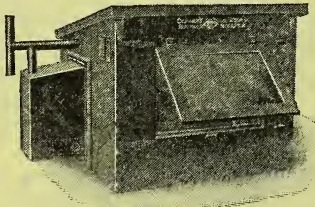
Cyphers "Style A" 2 Compartment Outdoor Brooder.
