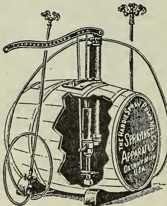
No. 6 Hardie Barrel Pump Mounted.
