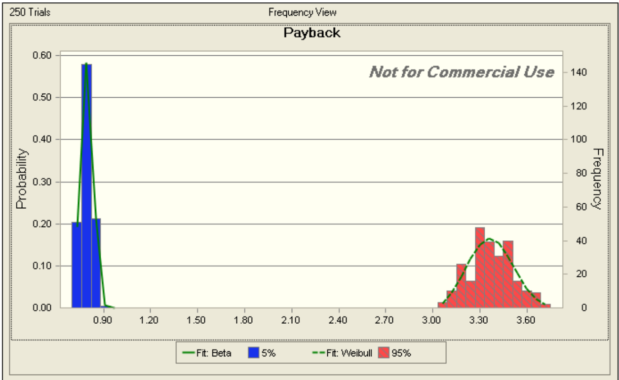
Figure 65. Scenario 17 Payback
