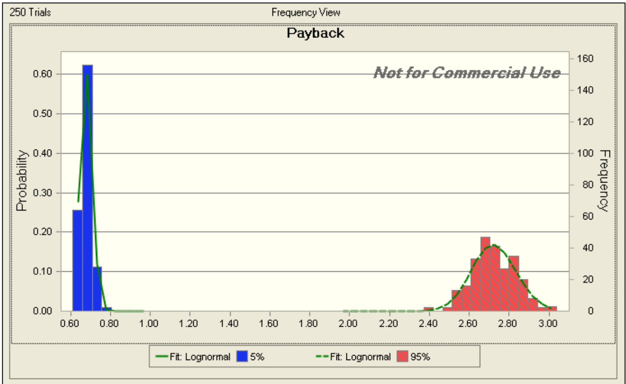
Figure 77. Scenario 21 Payback
