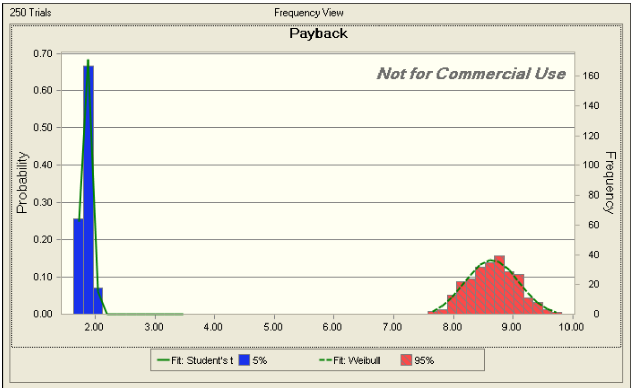
Figure 59. Scenario 15 Payback
