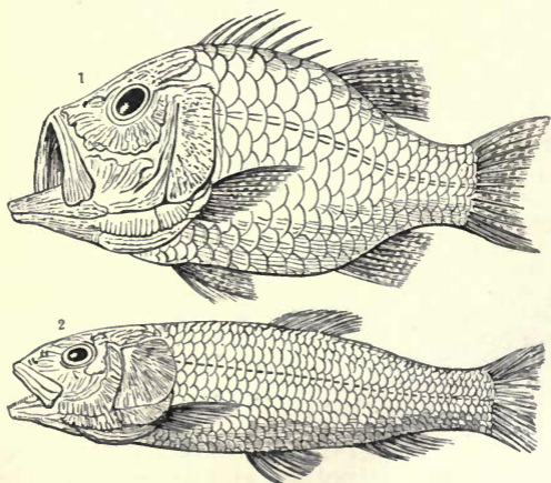
Fig. 279.—1. Beryx ( Osmeroides ) Lewesiensis , a Percoid fish from the Chalk; 2. Osmeroides Mantelli , a Salmonoid fish from the Chalk.
