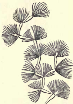
Fig. 27.— Oldhamia antiqua , natural size (after Salter). Cambrian.
