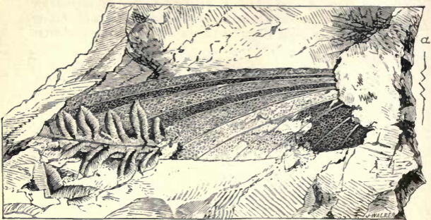
Fig. 129.— Haplophlebiium Barnesii (after Dawson). From the Carboniferous Rocks of Canada. a Profile of base of wing.
