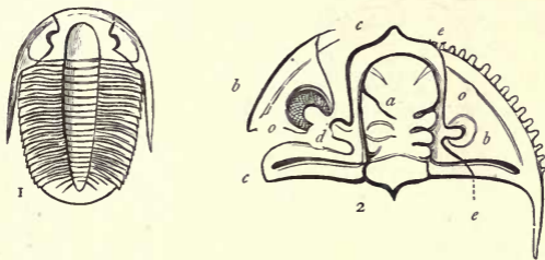
Fig. 103.—Morphology of Trilobites. 1. Angelina Sedgwickii , Upper Cambrian. 2. Diagram of a Trilobite (after Salter): a Glabella with its furrows; bb Free cheeks, bearing the eyes ( oo ); c c Fixed cheek, including the eye-lobe ( d ); e e Facial suture.
