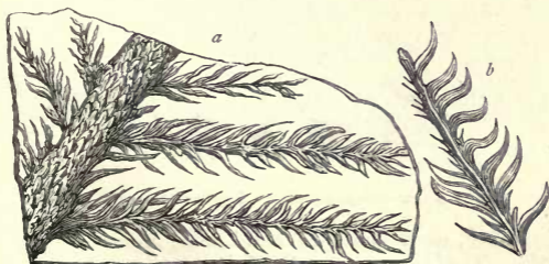
Fig. 391.— Walchia piniformis ; a Branch; b Twig. From the Permian of Saxony. (After Gutbier.)
