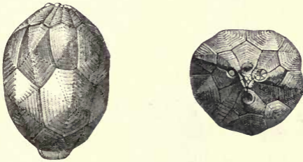
Fig. 82.— Hemicosmites pyriformis , one of the Cystideans. The right-hand figure shows the upper surface of the calyx.
