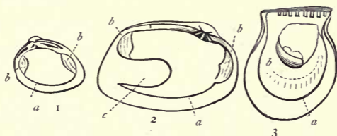
Fig. 168.—Shells of Lamellibranchiata. 1. Cyclas amnica , a dimyary shell with an entire pallial line. 2. Tapes fullastra , a dimyary shell with an indented pallial line. 3. Perna ephippium , a monomyary shell. (After Woodward.) a Pallial line; b Muscular impressions left by the adductors; c Siphonal impression.
