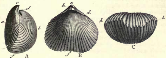
Fig. 139.— Rhynchonella sulcata . A, Profile view. B, View of the dorsal surface. C, View of the base. a Ventral valve; b Dorsal valve; f Base; c Beak; k Foramen. Lower Cretaceous.
