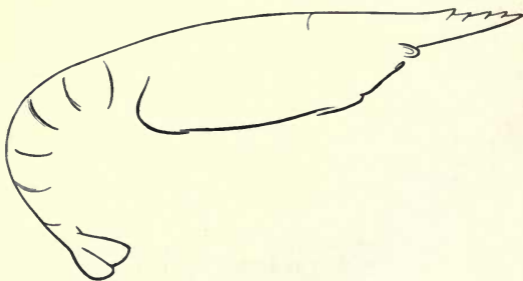
Fig. 121.— Anthropalemon Salteri , Carboniferous. (After Salter.)
