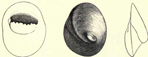
Fig. 219.— Nerita Schemidelliana . Eocene Tertiary.
