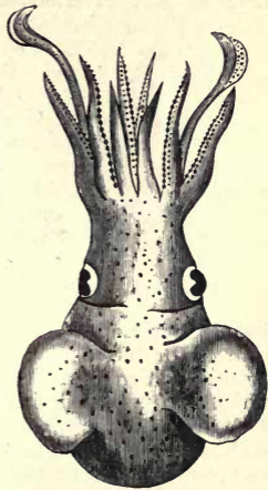
Fig. 246.—Cephalopoda. Sepiella Atlantica , one of the Cuttle-fishes (after Woodward).
