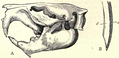
Fig. 371.—A, Skull of the Beaver (after Owen). B, Diagram of the incisor teeth of a Rodent, showing the chisel-shaped point: a Enamel; d Dentine.
