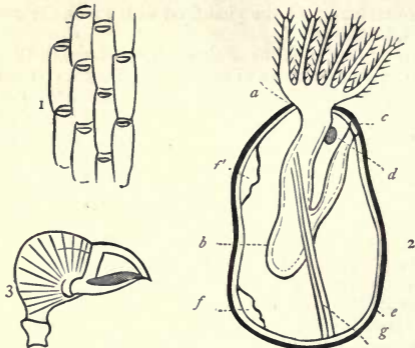
Fig. 131.—Morphology of Polyzoa. 1. Portion of the cœnœcium of Flustra truncata , magnified. 2. Diagram of a Polyzoön (after Allman): a Region of the mouth surrounded by tentacles; b Alimentary canal; c Anus; d Nervous ganglion; e Investing sac (ectocyst); f Testis; f' Ovary; g Retractor muscle. 3. Bird's-head process, or "avicularium," of a Polyzoön.
