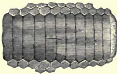
Fig. 305.—Teeth of a fossil Ray ( Myliobatis Edwardsii ). Eocene.
