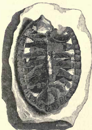
Fig. 314.— Chelone Benstedii . Lower Chalk.
