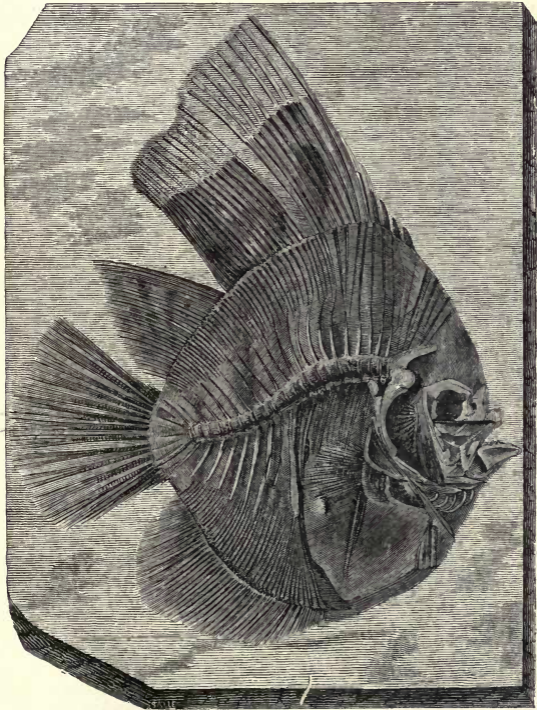
Fig. 281.— Platax altissimus , a Chetodont from the Eocene Tertiary of Monte Bolca.
