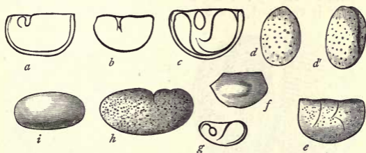
Fig. 100.—Fossil Ostracode Crustaceans:— a Primitia strangulata , Lower Silurian; b Primitia Logani , Lower Silurian; c Beyrichia Klædeni , Upper Silurian; d & d' Cytherella inflata , Carboniferous; e Leperditia Anna , Lower Silurian; f Leperditia Canadensis , Lower Silurian; g Beyrichia impendens , Upper Silurian; h Beyrichia subarcuata , Carboniferous; i Candona Tateana , Carboniferous. All enlarged.
