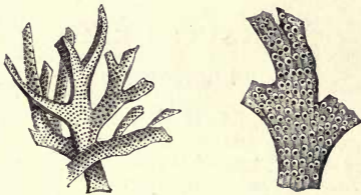
Fig. 136.— Bidiastopora cervicornis , natural size and enlarged. Oolites.
