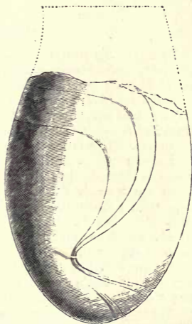
Fig. 256.— Ascoceras Canadensis (Billings), showing the form of the septa. Lower Silurian.
