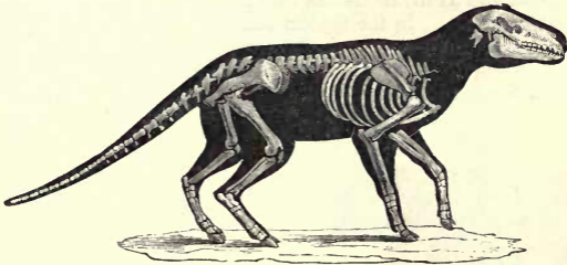
Fig. 354.— Anoplotherium commune . Eocene Tertiary.
