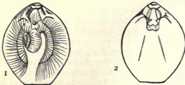
Fig. 138.—Brachiopoda.— Terebratulina vitrea . 1. Showing the ciliated "arms;" 2. Showing the shell with its loop. (After Woodward.)
