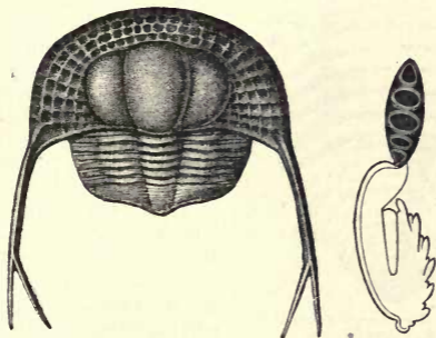
Fig. 115.— Trinucleus Pongervardi , Lower Silurian.
