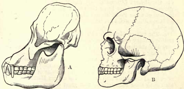
Fig. 377.—A, Skull of the Orang-utang. B, Skull of an adult European.
