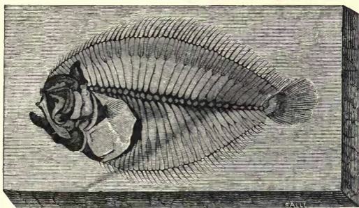
Fig. 280.— Rhombus minimus . A small fossil Turbot from the Eocene Tertiary of Monte Polca.
