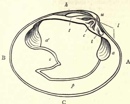
Fig. 167.—Left valve of Cytherea chione (after Woodward). A, Anterior margin; B, Posterior margin; C, Ventral margin or base; u Umbo; h Ligament; l Lunule; c Cardinal tooth; t t' Lateral teeth; a Anterior adductor; a' Posterior adductor; p Pallial line; s Pallial sinus, caused by the retractor muscles of the siphons.
