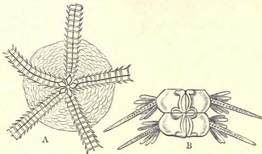
Fig. 70.— Protaster Sedgwickii . Upper Silurian. A, Disc and bases of the arms, magnified. B, Portion of an arm greatly enlarged.
