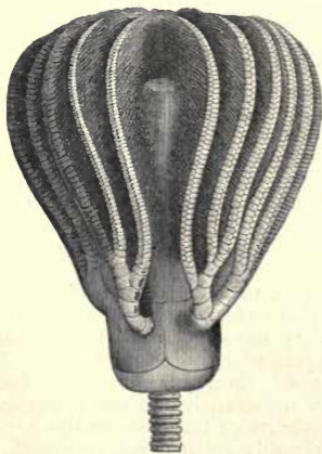
Fig. 73.— Platyrrhinus tricontadactylus . Carboniferous. The left-hand figure shows the calyx, arms, and upper part of the stem, and the figure next this shows the surface of one of the joints of the column. The right-hand figure shows the proboscis; and above is a magnified figure of part of one arm with its pinnulæ.
