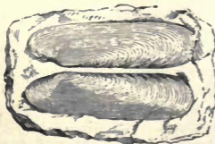
Fig. 182.— Orthonota parvella . Lower Silurian.
