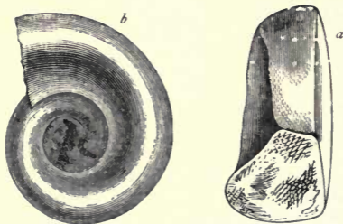
Fig. 221.— Euomphalus De Cevi (Billings). a Front view; b View of the umbilicus. Devonian.
