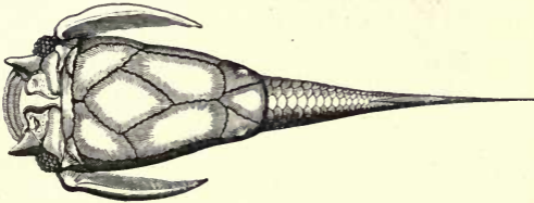
Fig. 294.— Pterichthys cornutus . Old Red Sandstone.
