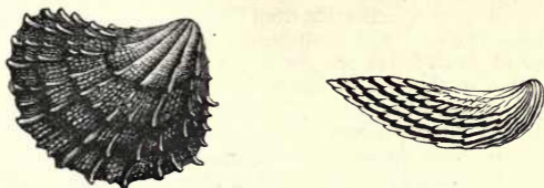
Fig. 175.— Plicatula placunea , Lower Greensand.
