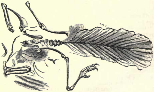
Fig. 333.— Archæopteryx macrura , showing tail and tail-feathers, with detached bones.
