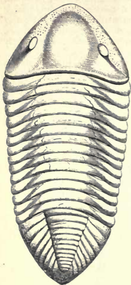
Fig. 116.— Homalonus delphinocephalus , Upper Silurian.
