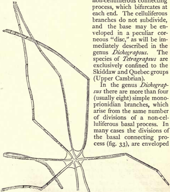
Fig. 33.— Dichograpsus octobrachiatus , showing the central disc (after Hall). Skiddaw and Quebec groups.
