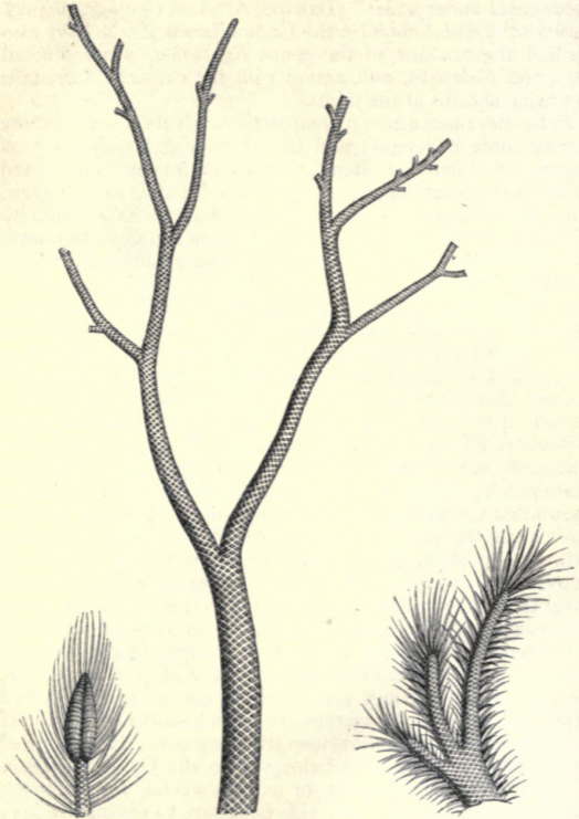
Fig. 387.— Lepidodendron Sternbergii . Carboniferous.
