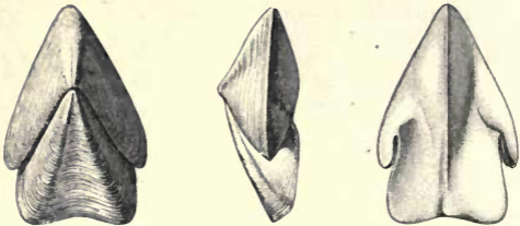
Fig. 247.— Rhynchoteuthis Astieriana . Lower Greensand (Cretaceous).
