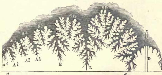
Fig. 257.—One-half of the suture of Ammonites Truelli . D, Dorsal lobe, traversed by the siphuncle; L, Lateral-superior lobe; E, Lateral-inferior lobe; A^1 , A^2 , A^3 , A^4 , Auxiliary lobes; SD, Dorsal saddle; SL, Lateral saddle; S^1 , S^2 , S^3 , S^4 , Auxiliary saddles.
