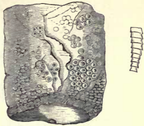
Fig. 88.— Conchicolites gregarius , growing upon the shell of an Orthoceras . Lower Silurian.
