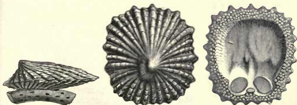
Fig. 161.— Crania Ignabergensis , Cretaceous.
