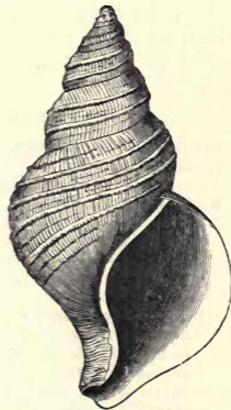
Fig. 206.— Fusus tornatus , a Siphonostomatous Univalve. Post-Pliocene.
