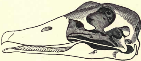
Fig. 328.—Skull of Spur-winged Goose ( Plectropterus Gambensis ).
