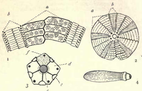
Fig. 57.—Morphology of Echinoidea. 1. Portion of the test of Galerites hemisphericus enlarged, showing an inter-ambulacral area ( a ), and an ambulacral area ( b ). 2. Galerites hemisphericus viewed from above. a Inter-ambulacra; b Ambulacra. 3. Genital and ocular disc of Hemicidaris intermedia enlarged. c Ocular plate; d Genital plate; e Anal aperture; f Madreporiform tubercle. 4. Spine of the same. (After Forbes.) The tubercles are mostly omitted on figs 2 and 3 for the sake of clearness.
