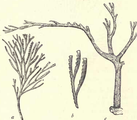
Fig. 25— Dendrograpsus Hallianus . a Portion of the frond, natural size; b Portion of a branch, enlarged; c The footstalk and some of the principal branches, natural size. (After Hall.)
