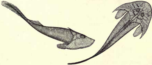
Fig. 292.— Cephalaspis Lyellii . (After Page.) Old Red Sandstone.
