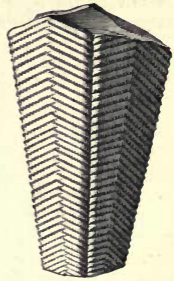
Fig. 244.— Conularia ornata . Devonian.
