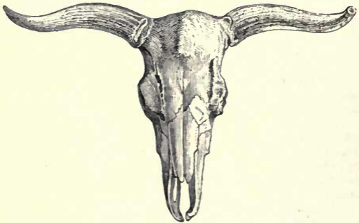
Fig. 358.—Skull of the Urus ( Bos primigenius ). Post-Pliocene and Recent.
