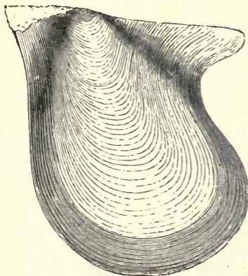
Fig. 176.— Avicula demissa , Lower Silurian.
