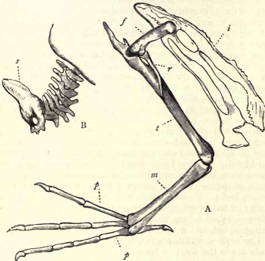
Fig. 330.—A, Hind-limb of the Loon ( Colymbus glacialis )—after Owen: i Innominate bone; f Thigh-bone or femur; t Tibia, with the proximal portion of the tarsus anchylosed with its lower end; r Fibula; m Tarso-metatarsus, consisting of the distal portion of the tarsus anchylosed with the metatarsus; p p Phalanges of the toes. B, Tail of the Golden Eagle: s Ploughshare-bone, carrying the great tail-feathers.
