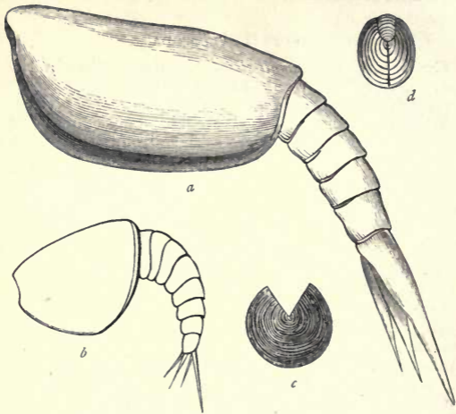
Fig. 102.—Paleozoic Phyllopods:— a Ceratiocaris papilio , Upper Silurian (Salter). b Hymenocaris vermicauda , Upper Cambrian (Salter). c Discinocaris Browniana , Lower Silurian (Original). d Peltocaris aptychoides , Lower Silurian (Woodward).
