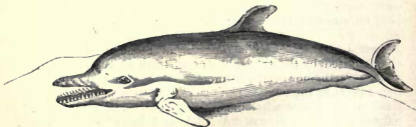
Fig. 348.—The common Dolphin ( Delphinus delphis ).
