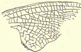
Fig. 128.—Wing of Platephemera antiqua (after Dawson), Devonian.
