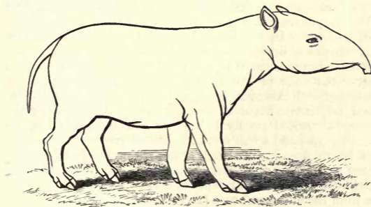
Fig. 352.—Outline of Palæotherium magnum , restored, after Cuvier. Upper Eocene.
