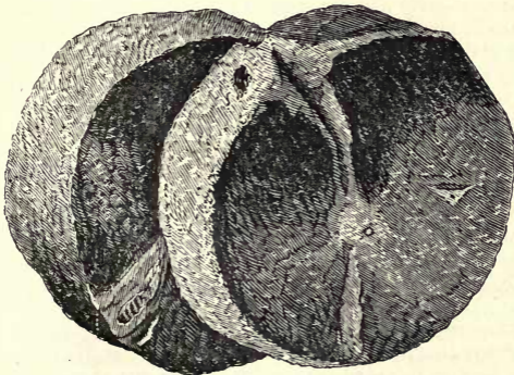
Fig. 320.—Two vertebrae of Eosaurus Acadiensis (Marsh). Coal-measures of Nova Scotia. (After Dawson.)
