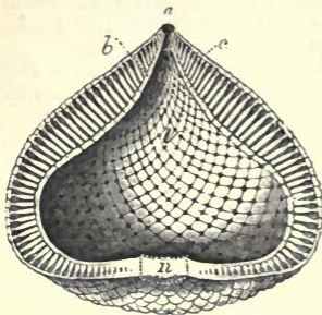
Fig. 20.—Diagram of the structure of Receptaculites , as it would be shown by a vertical section of a perfect specimen. a The aperture at the summit; b The inner integument; c The outer integument; n The usual position of the nucleus; v The great internal cavity. The unshaded bands running from the outer to the inner integument represent the tubes. (After Billings.)
