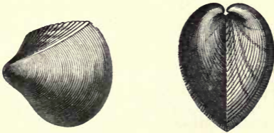
Fig. 192.— Cardium Hillanum . Upper Greensand.
