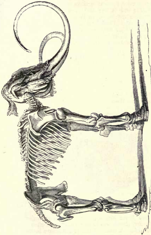
Fig. 363.—Skeleton of the Mammoth ( Elephas primigenius ). Post-Pliocene.
