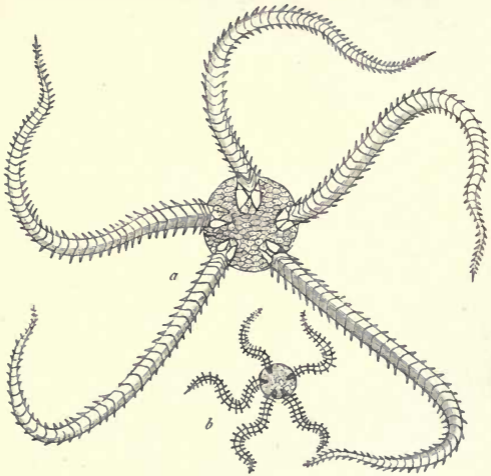
Fig. 69.—Recent Ophiuroids. a Ophiura texturata , the common Sand-star ; b Ophiocoma neglecta , the grey Brittle-star (after Forbes).
