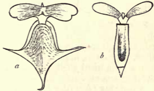
Fig. 241.—Pteropoda. a Cleodora pyramidata ; b Cuvieria columnella . (After Woodward.)
