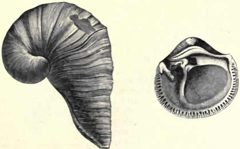
Fig. 191.— Caprina Aguilloni . The right-hand figure shows the interior of the left valve.
