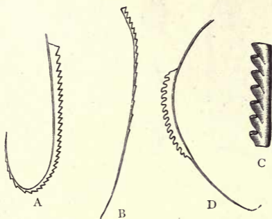
Fig. 29.—A, Young individual of Graptolites sagittarius , His., showing the slender curved base of the frond, and the extension of the axis beyond its opposite end; B, Base of another individual of the same, in which there is an extremely long "radicle;" C, Fragment of G. sagittarius , much enlarged to show the cellules—from a specimen in relief; D, Specimen of Graptolites Clingani , Carr., showing the distal and proximal extensions of the axis.
