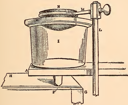
FIG. II. CROOKES' APPARATUS.
