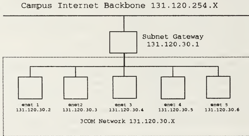
Figure 3.2 Subnetting
