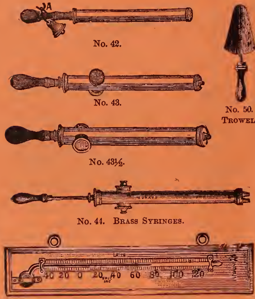
No. 45. MINIMUM REGISTERING THERMOMETER.
