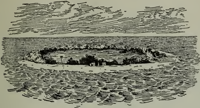
CORAL ISLAND.
