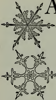
SNOW CRYSTALS.
