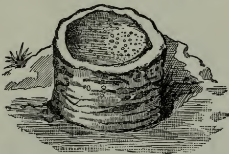
FIG. 1. CALCAREOUS CONCRETION SIMULATING A FOSSIL PALM-STEM, BOAZ ISLAND, BERMUDAS.
