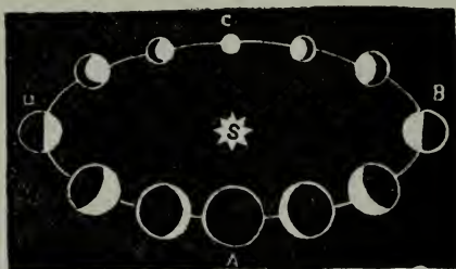
THE PHASES OF VENUS.
