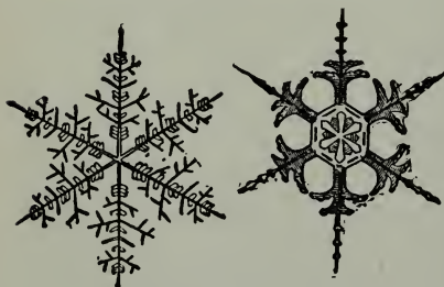
SNOW CRYSTALS.
