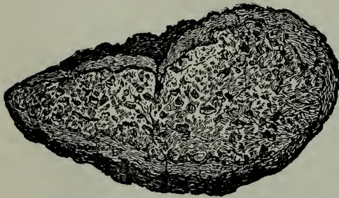
SECTION OF A LAVA BOMB.
