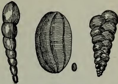
RHIZOPODS (MAGNIFIED).
