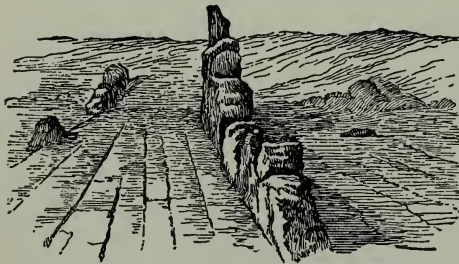
DIKES.
