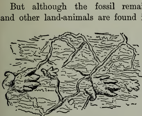
FOSSIL FOOTPRINTS.
