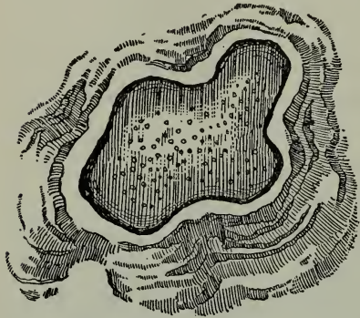
FIG. 2. CALCAREOUS CONCRETION IN AEOLIAN LIMESTONE, BERMUDAS.
