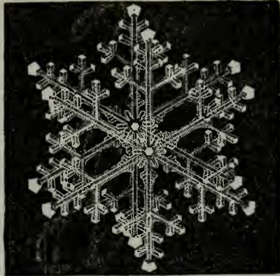
SNOW-STAR.
