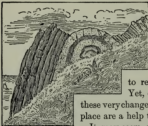
EXAMPLE OF DISTURBANCE OF THE EARTH'S LAYERS.
