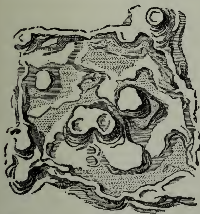
FIG. 5. CALCAREOUS CONCRETION IN AEOLIAN LIMESTONE, BERMUDAS.
