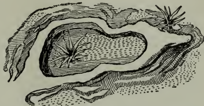
FIG. 4. CALCAREOUS CONCRETION, BERMUDAS.
