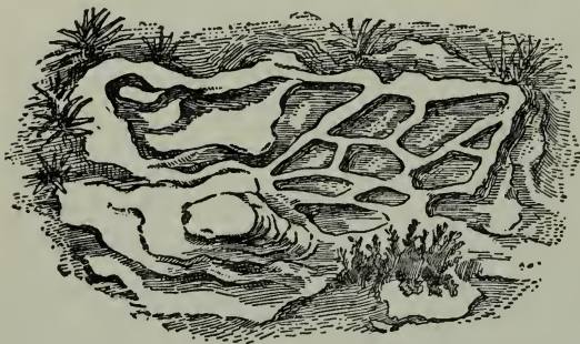
FIG. 6. CONCRETIONS IN AEOLIAN ROCKS, BERMUDAS.
