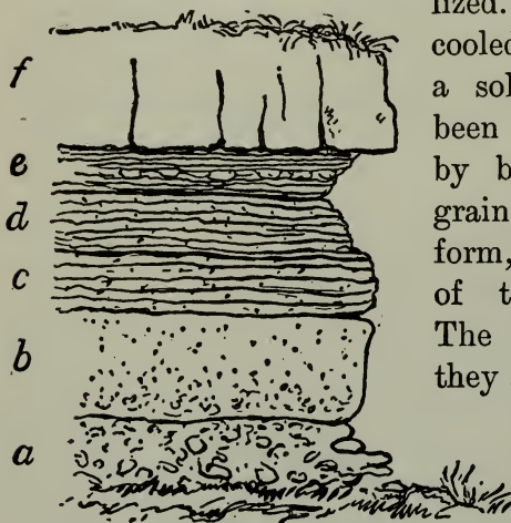
SECTION OF STRATIFIED ROCKS.
