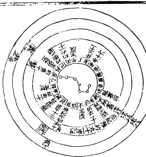
斗綱所指月建圖
