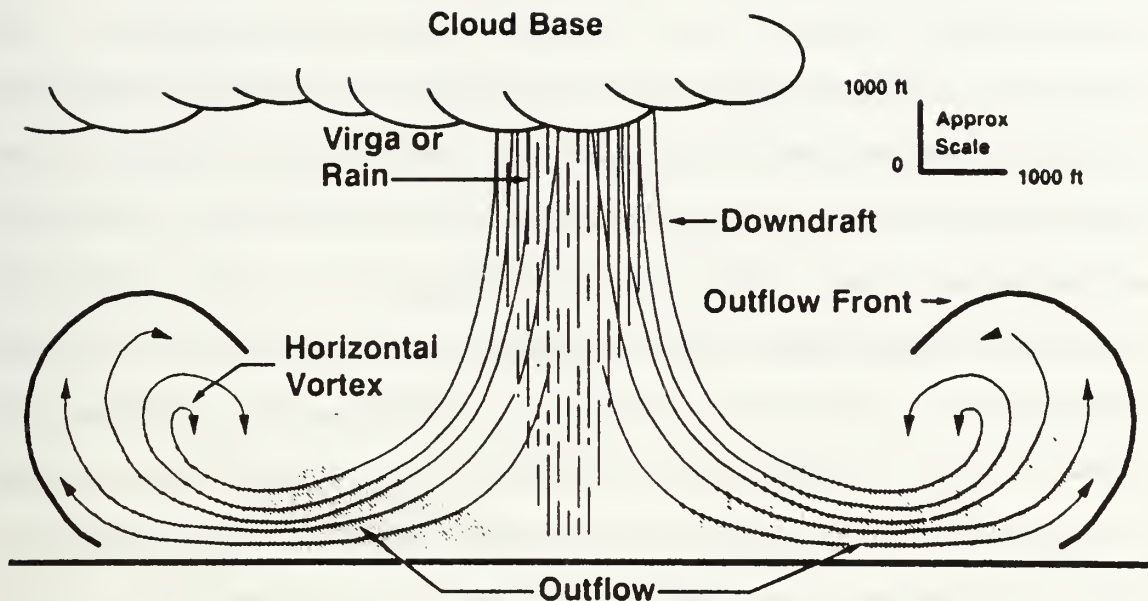
Figure 1. Symmetrical microburst
