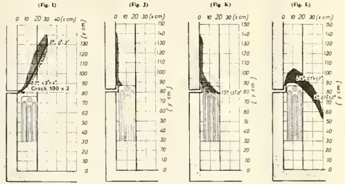
Fig. 4 Test Results with an Air Flow of 60 Cubic Meters Per Hour Vertical project of discomfort zone and indicator of maximum values of \rho_{g, \text{air}} and \Delta t_{\text{air}} along the air stream.
