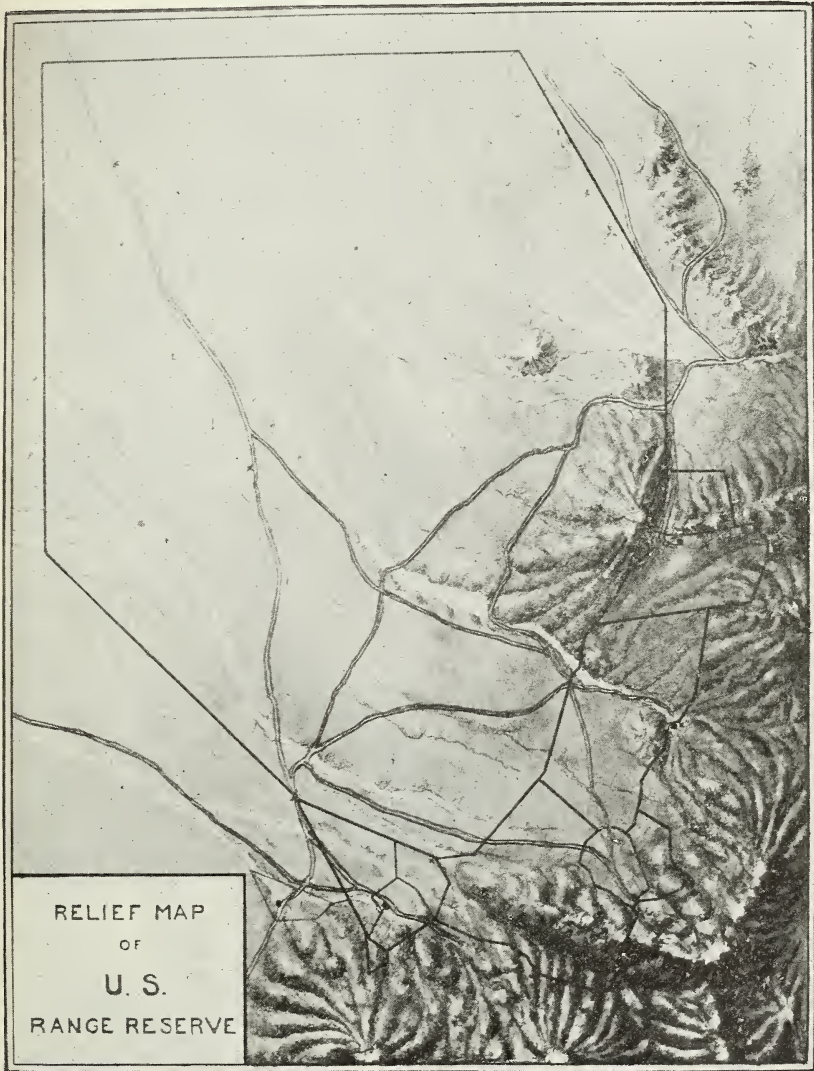
FIG. 1.—Relief map of the Santa Rita Range Reserve, Ariz., and some of the territory immediately surrounding it.
