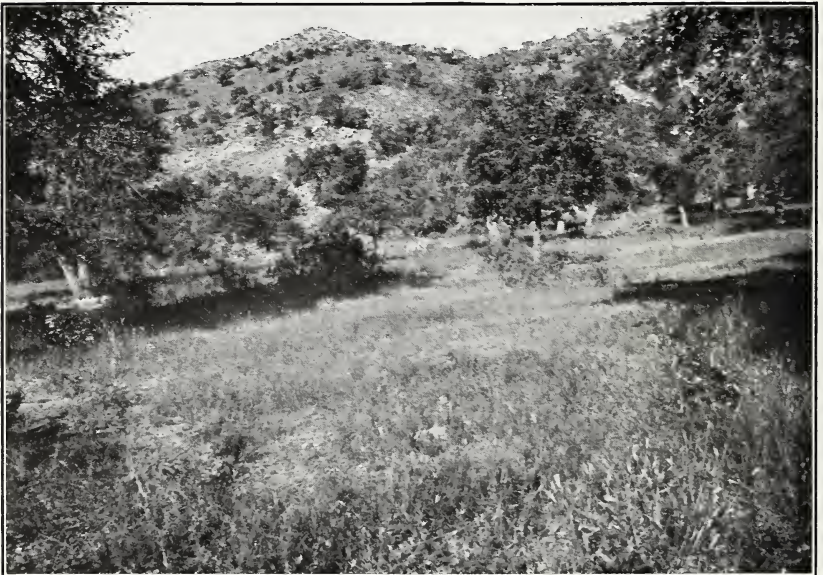
FIG. 2.—GRAZING CONDITIONS IN THE OAK BELT ON THE RESERVE.
