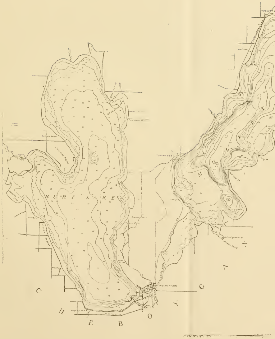
Fig. 37. Map showing outlines and configuration of the bottom of Burt and Mullet Lakes. (After U. S. Lake Survey Chart.)
