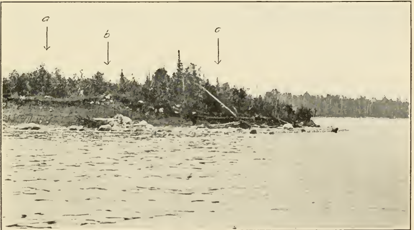
B. STONEY POINT, MULLETT LAKE. a, NIPISSING TERRACE, b, ICE RAMPART, c, POST-NIPISSING TERRACE.
