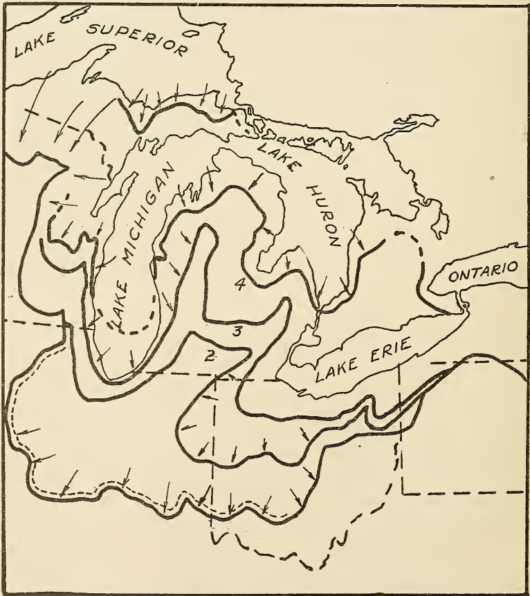
Fig. 3. Map of the principal moranic systems of Michigan. On this map are shown the southern limits of the Wisconsin stage of glaciation; 2, the Kalamazoo-Mississinawa moranic system; 3, the Valpariso-Charlotte moranic system; 4, Port Huron moranic system.
