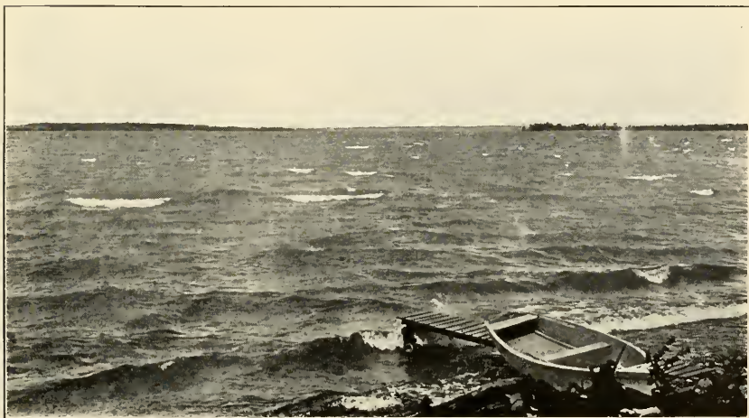
B. WHITECAPS AND BREAKERS, HIGGINS LAKE.
