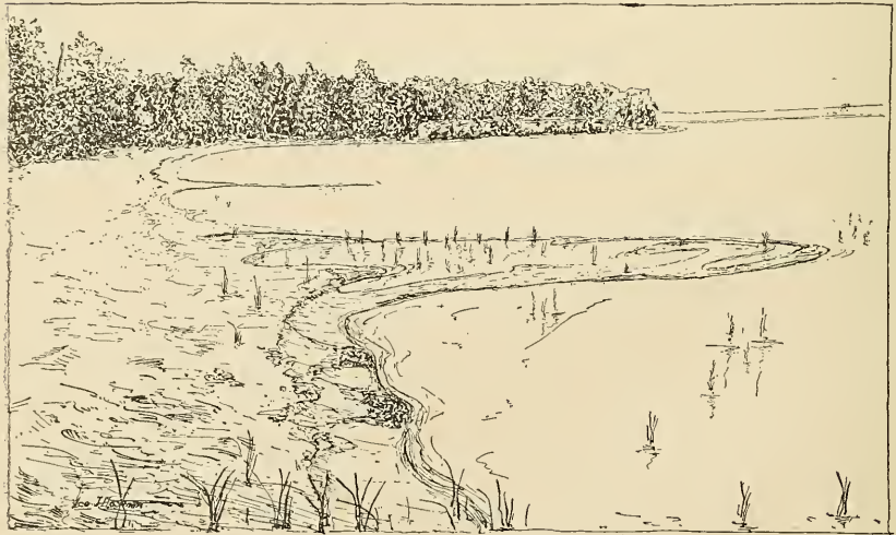
Fig. 44. Sand cusp, Douglass Lake.
