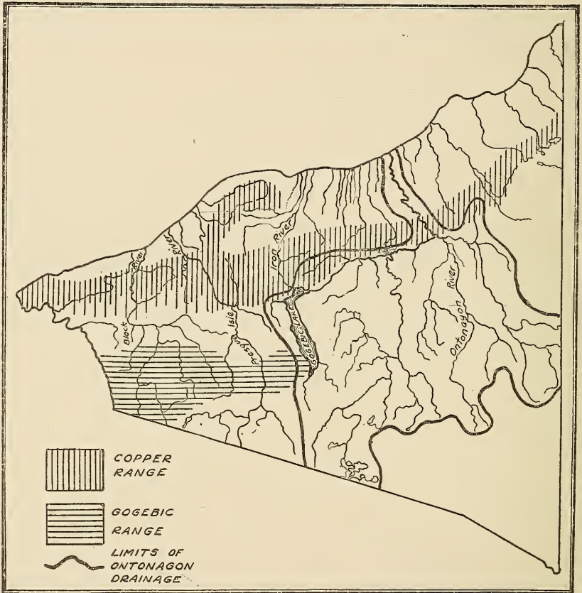
Fig. 91. Map of western part of the Northern Peninsula showing the general distribution of the Copper and Gogebic Ranges and also the basin of the Ontonagon River.
