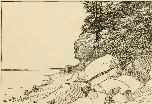
Fig. 26. Farwell's Point, an undercut notched cliff on Lake Mendota, Wisconsin. After a time the overhanging portion will fall by gravity to produce blocks like those in the foreground, (after Fenneman).
