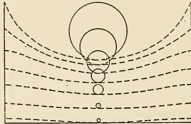
Fig. 18. Diagram illustrating rapid decrease, with depth, of motion of water particles in a wave, (after Penniman).
