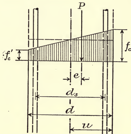
FIG. 59.—Column with Eccentric Load.
