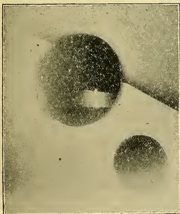
FIG. 2. SHOWING REFLECTION AND INTERFERENCE OF X-RAYS.
