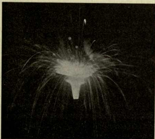
FIG. 83.—Photograph of the combustion of an iron wire in a spoon. The spoon can be dimly seen. Below it is the flame of a Bunsen burner. The white lines show the paths of particles of burning iron.
