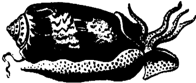
Fig. 759.—Olive-Shell ( Oliva )
