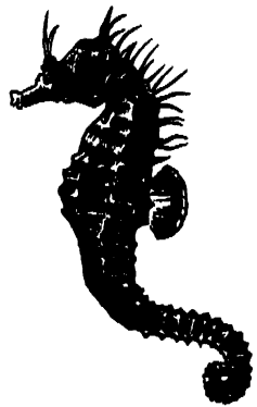
Fig. 615.—Sea-Horse ( Hippocampus )
