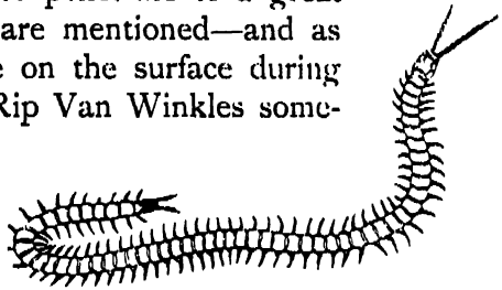
Fig. 771.—Earth-Centipede ( Geophilus )
