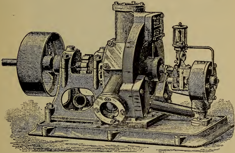
STATIONARY ENGINE.
