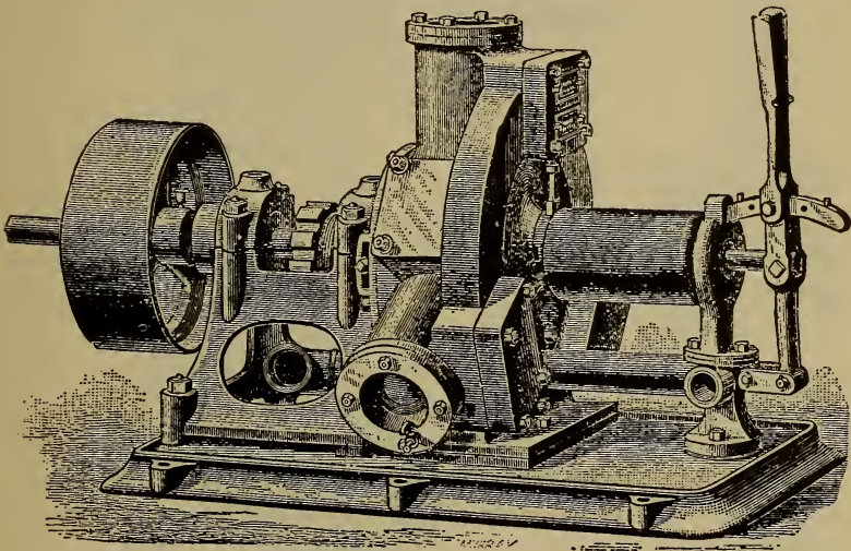
EVERSING ENGINE.
