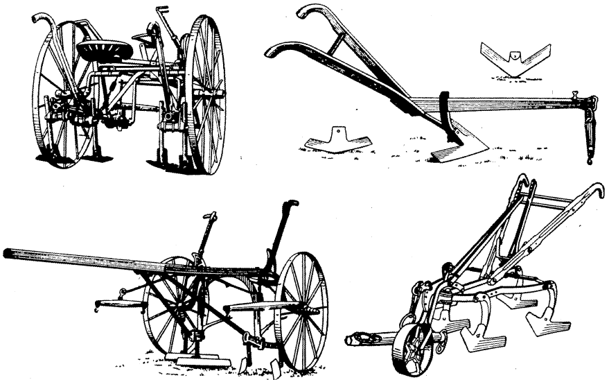
FIG. 22.—Various types of cultivators equipped with knives or sweeps that are effective in cutting off the stems of perennial weeds below the soil surface.
