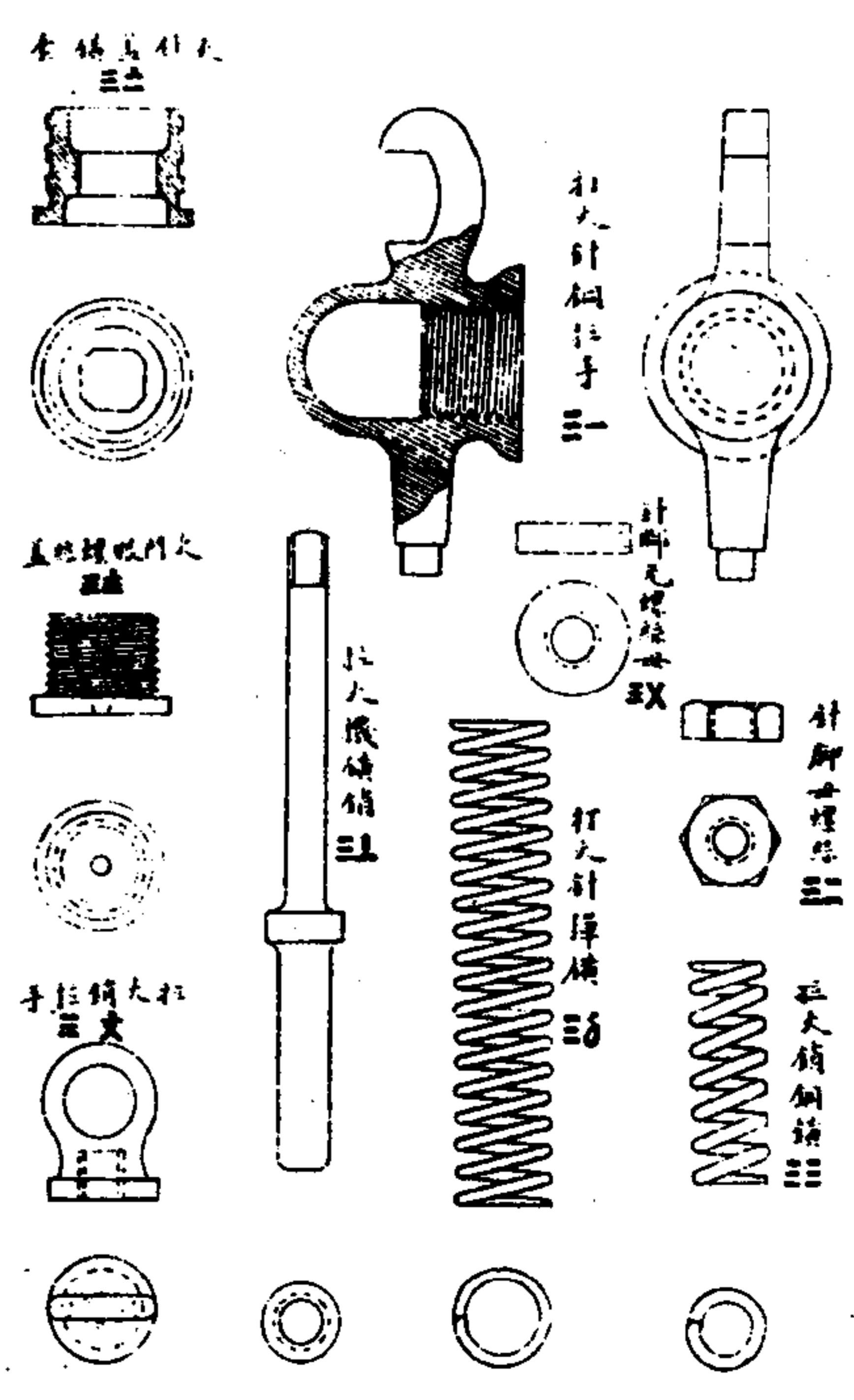
破圖十
