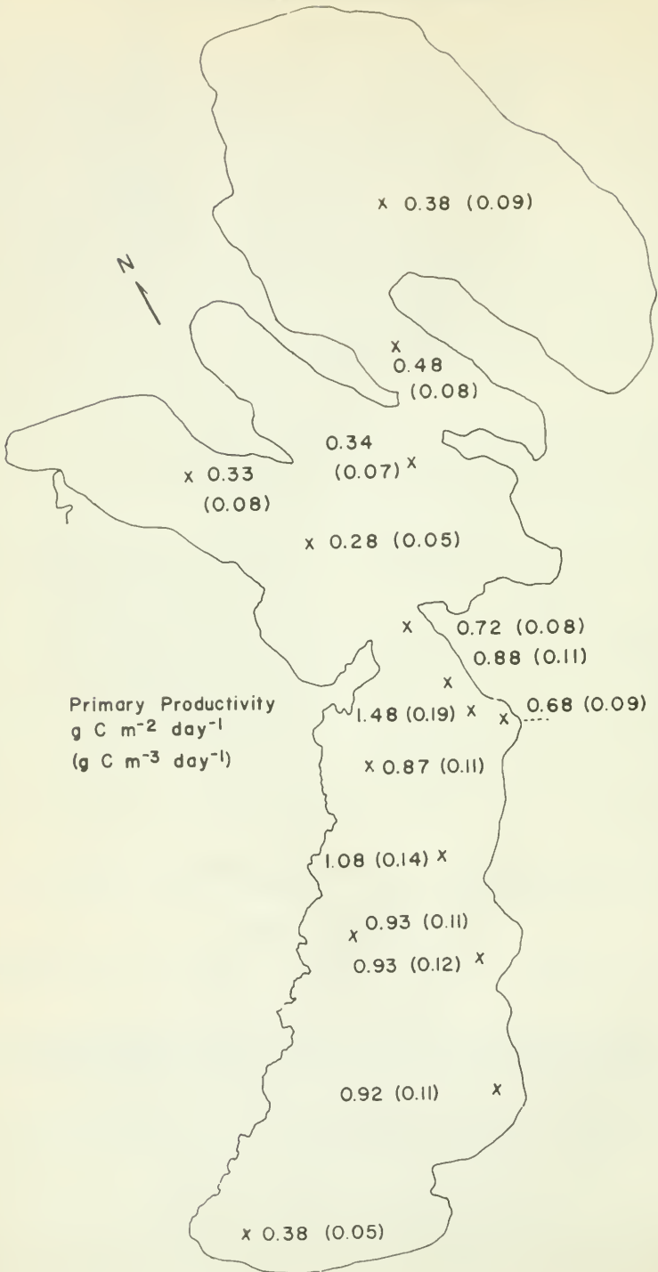
FIGURE 5. Distribution of phytoplankton production in Eagle Lake during mid-July through mid-August 1971.
