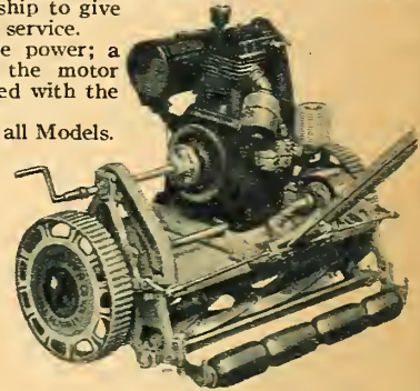
Super Detroit
