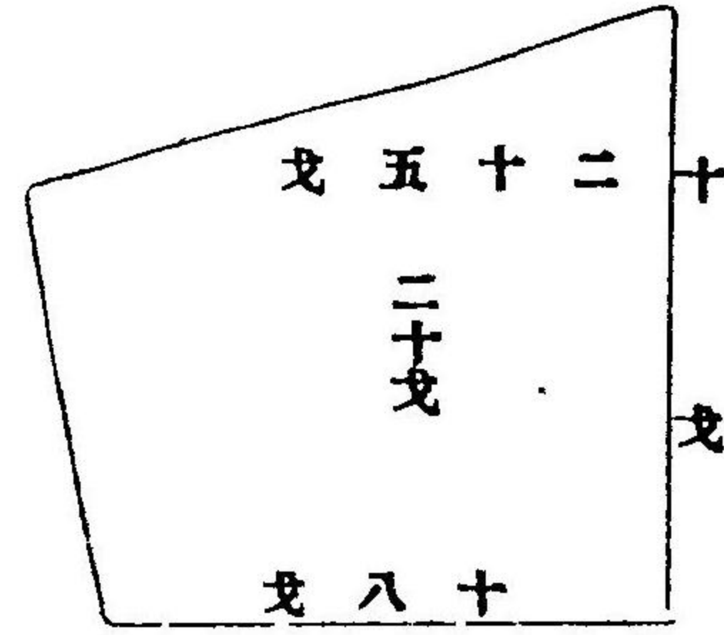
斜併股勾
