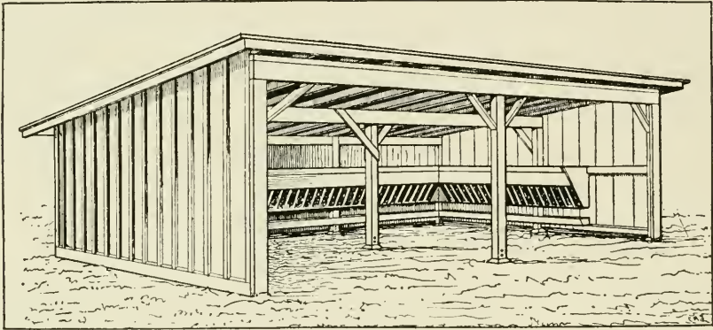
This Shed Can Be Used When Feeding in an Open Lot. It Should be Open to the Sun. It is Inexpensive and Can Be Made in Any Length or Width
