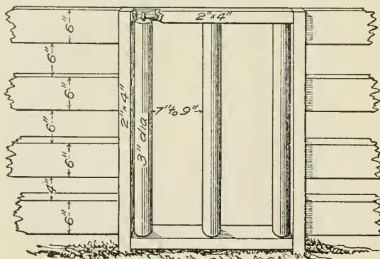
Lamb creep with rollers for uprights
