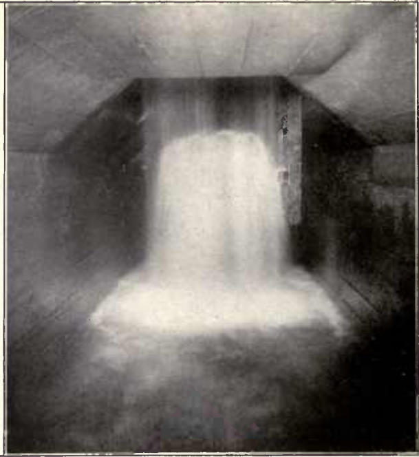
JUNCTION OF THE GALLERIES, SUNOL.
