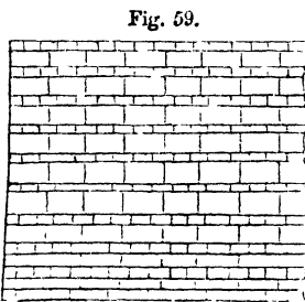
Fig. 59 shows the elevation of a wall so constructed. The advantages of hollow walls are a saving of one-third of the number of bricks, as 4500 are required for a rod of reduced brickwork, according to the usual mode of building;
